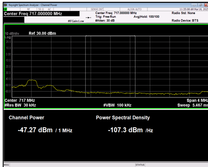
Band17 16QAM BW=10MHz Channel=23800 RB Size=1 Position=#Max Extended
