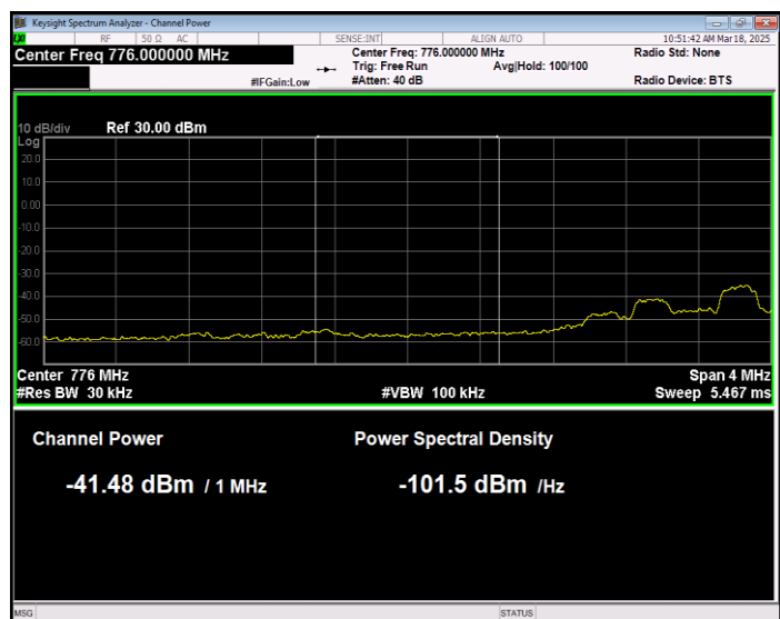
Band13 QPSK BW=5MHz Channel=23205 RB Size=25 Position=#0 Extended
