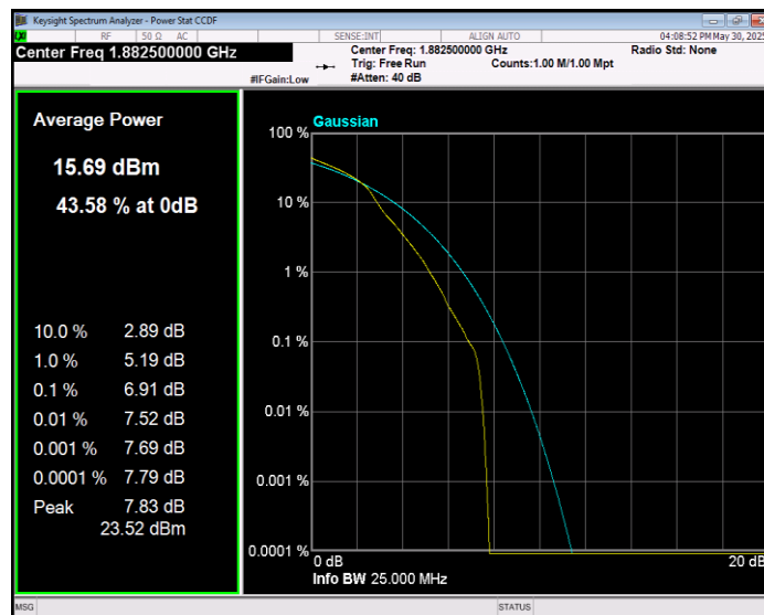
Band25 16QAM BW=3MHz Channel=26675 RB Size=1 Position=#0
