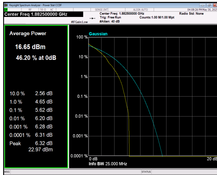
Band25 QPSK BW=1.4MHz Channel=26683 RB Size=1 Position=#0
