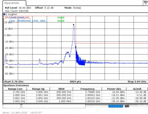
n78(3700-3800) SCS=30kHz DFT_QPSK BW=40MHz HighChannel=652000 RB=1@105
