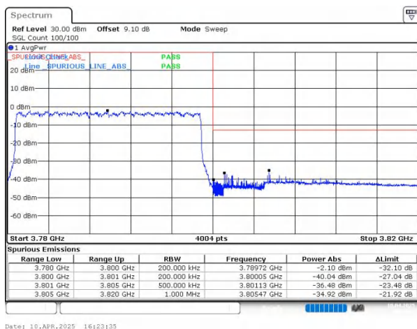
n78(3700-3800) SCS=30kHz DFT_256QAM BW=20MHz HighChannel=652666 RB=50@0
