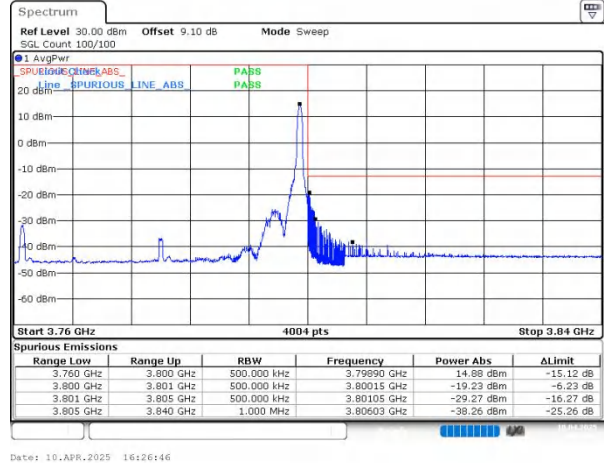
n78(3700-3800) SCS=30kHz DFT_256QAM BW=40MHz HighChannel=652000 RB=1@105
