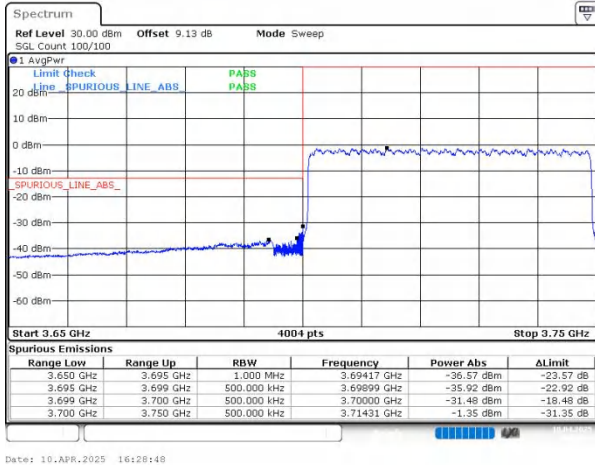
n78(3700-3800) SCS=30kHz CP_QPSK BW=50MHz LowChannel=648334 RB=133@0
