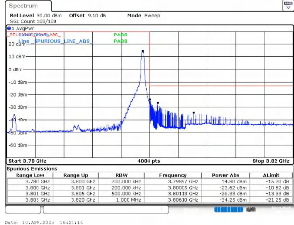
n78(3700-3800) SCS=30kHz DFT_BPSK BW=20MHz HighChannel=652666 RB=1@50
