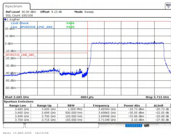
n78(3700-3800) SCS=30kHz DFT_BPSK BW=15MHz LowChannel=647168 RB=36@0
