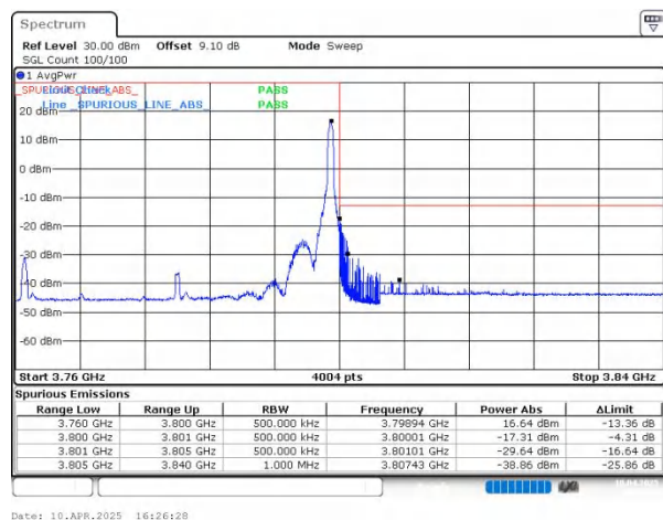
n78(3700-3800) SCS=30kHz DFT_64QAM BW=40MHz HighChannel=652000 RB=1@105
