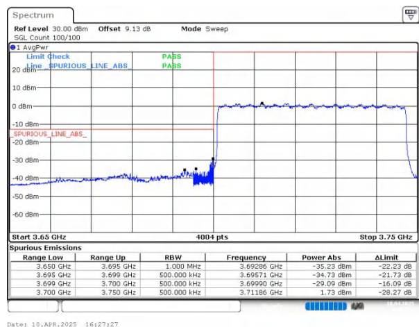
n78(3700-3800) SCS=30kHz DFT_BPSK BW=50MHz LowChannel=648334 RB=128@0
