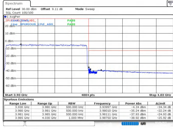
n77(3700-3980) SCS=30kHz CP_QPSK BW=50MHz HighChannel=663666 RB=133@0
