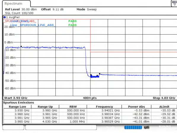
n77(3700-3980) SCS=30kHz DFT_256QAM BW=50MHz HighChannel=663666 RB=128@0
