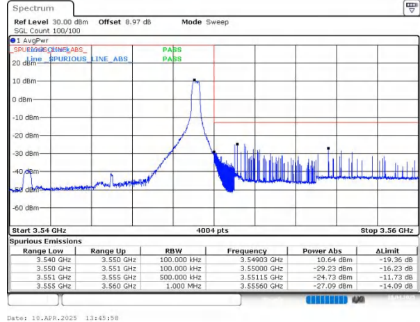
n78(3450-3550) SCS=30kHz DFT_256QAM BW=10MHz HighChannel=636332 RB=1@23
