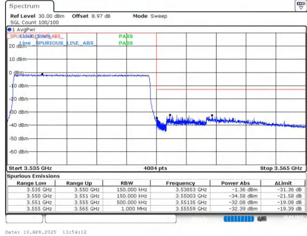
n78(3450-3550) SCS=30kHz CP_QPSK BW=15MHz HighChannel=636166 RB=38@0
