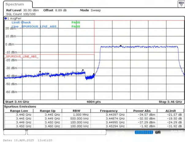
n78(3450-3550) SCS=30kHz DFT_256QAM BW=10MHz LowChannel=630334 RB=24@0
