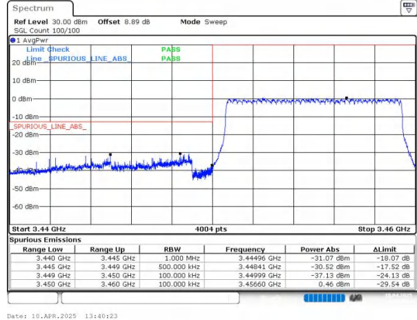
n78(3450-3550) SCS=30kHz DFT_64QAM BW=10MHz LowChannel=630334 RB=24@0
