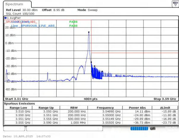
n78(3450-3550) SCS=30kHz DFT_16QAM BW=40MHz HighChannel=635332 RB=1@105
