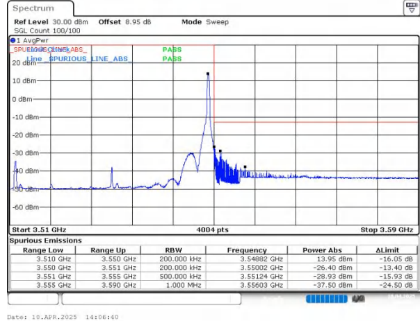
n78(3450-3550) SCS=30kHz DFT_QPSK BW=40MHz HighChannel=635332 RB=1@105
