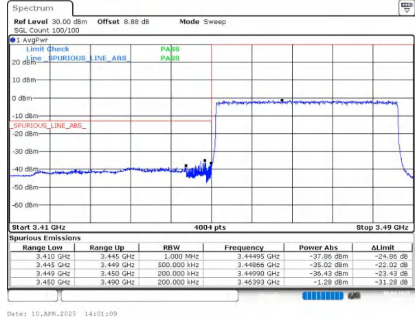
n78(3450-3550) SCS=30kHz DFT_BPSK BW=40MHz LowChannel=631334 RB=100@0
