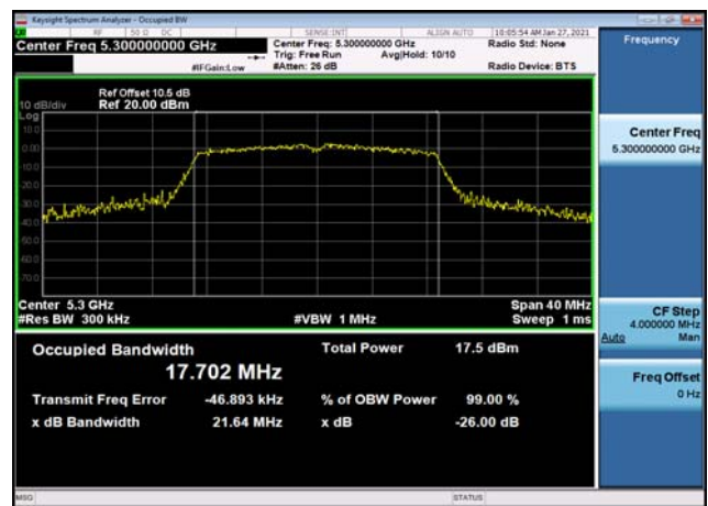
U-NII-2a 99% Bandwidth-802.11ac(20MHz) ,5300MHz,Ant1
