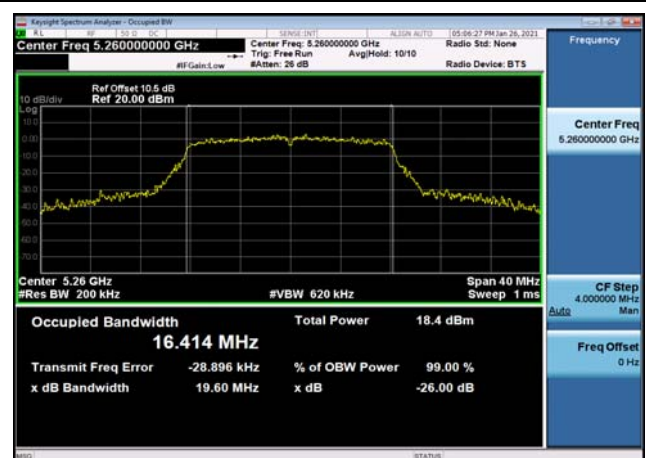
U-NII-2a 26dB Bandwidth-802.11a(20MHz )5260MHz,Ant1
