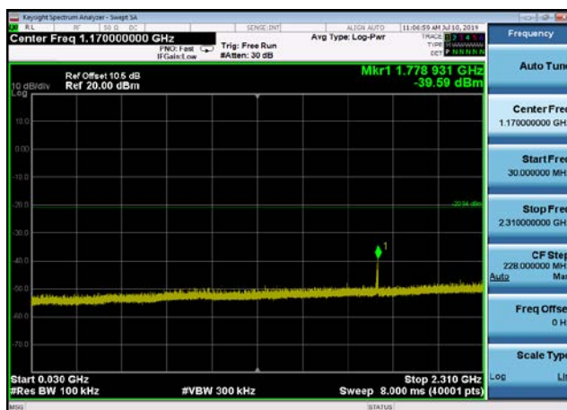
,Plot 3,30MHz~2310MHz-802.11g,2462MHz
