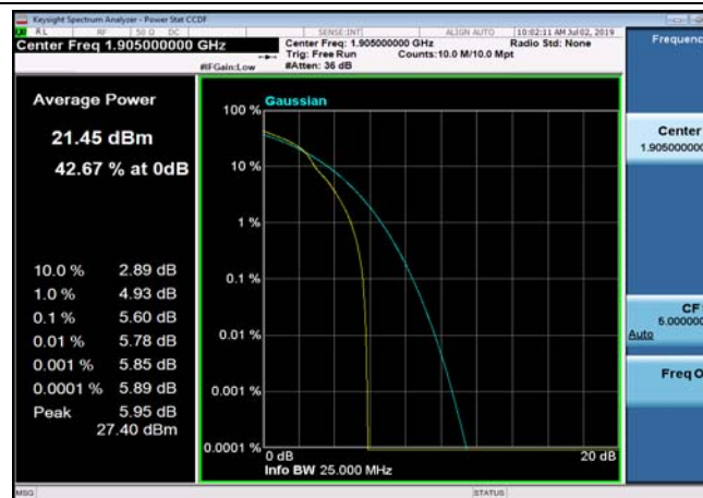
FDD25_HighRange_20MHz_1905_OneRB _high_Q16
