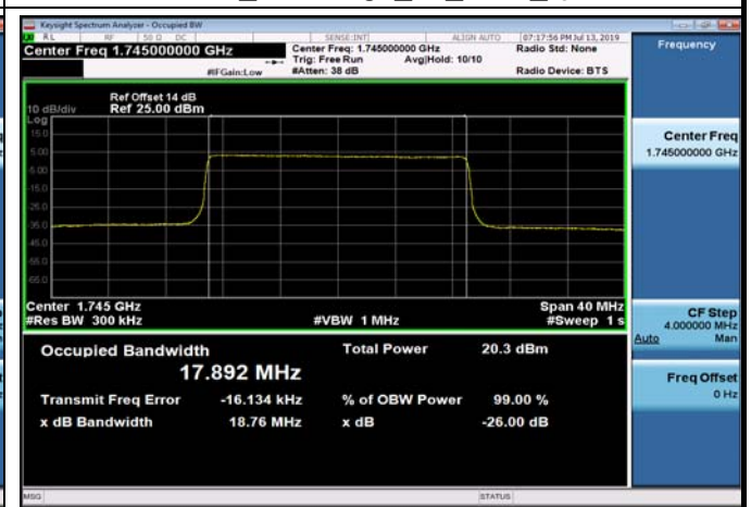
FDD66_MidRange_20_1745_Q16
