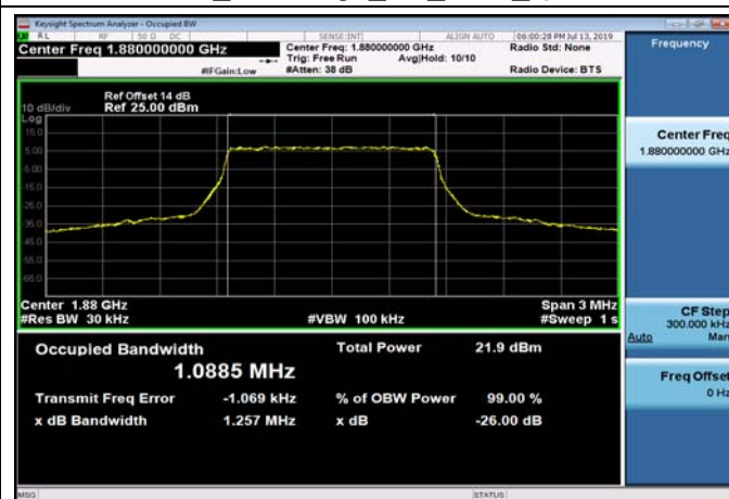
FDD02_MidRange_3_1880_QPSK
