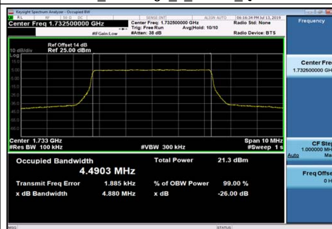
FDD04_MidRange_5_1732.5_QPSK
