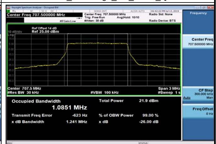
FDD12_MidRange_1.4_707.5_Q16
