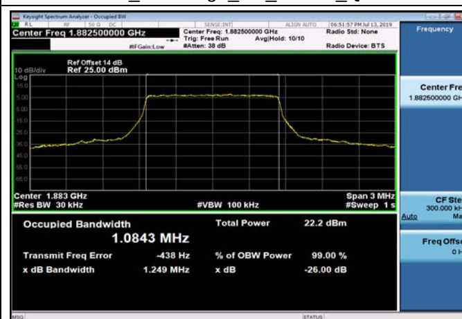
FDD25_MidRange_1.4_1882.5_QPSK
