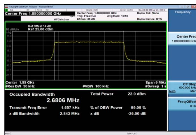
FDD02_MidRange_5_1880_QPSK
