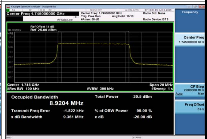
FDD66_MidRange_10_1745_Q16
