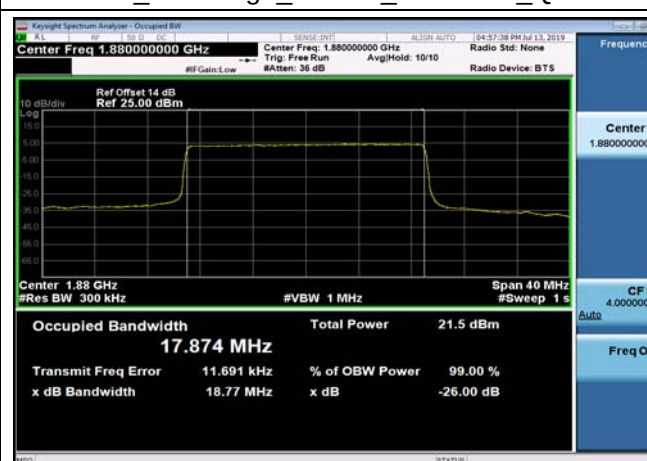
FDD02_MidRange_20MHz_1880MHz_QPSK
