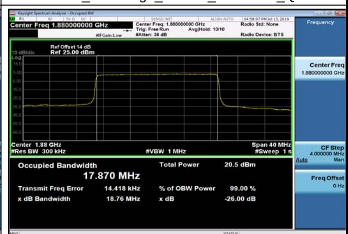
FDD02_MidRange_20MHz_1880MHz_Q16
