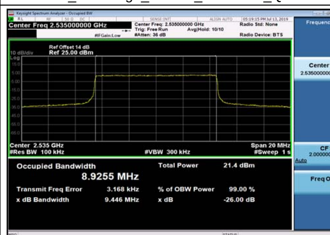
FDD07_MidRange_10MHz_2535MHz_QPSK
