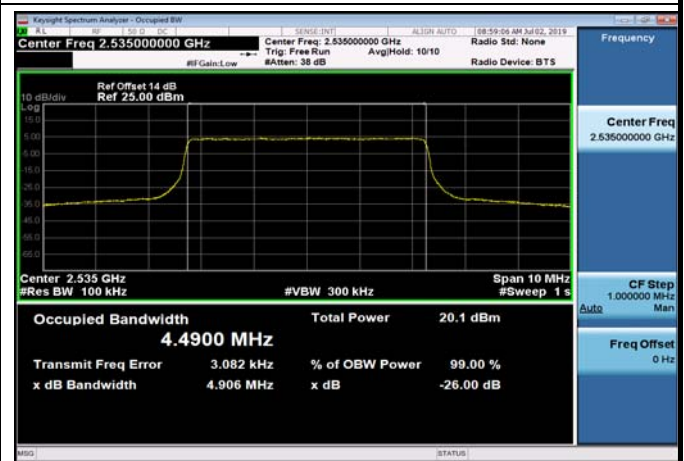
FDD07_MidRange_10_2535_Q16
