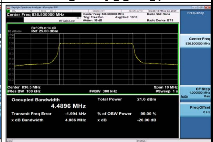
FDD05_MidRange_5_836.5_Q16
