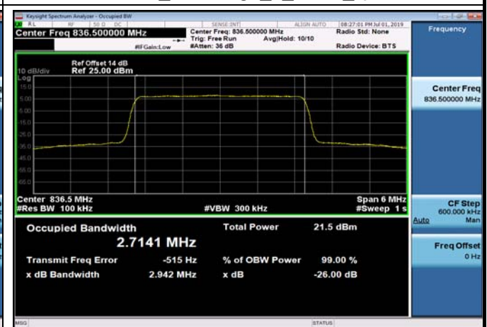
FDD05_MidRange_5_836.5_Q16
