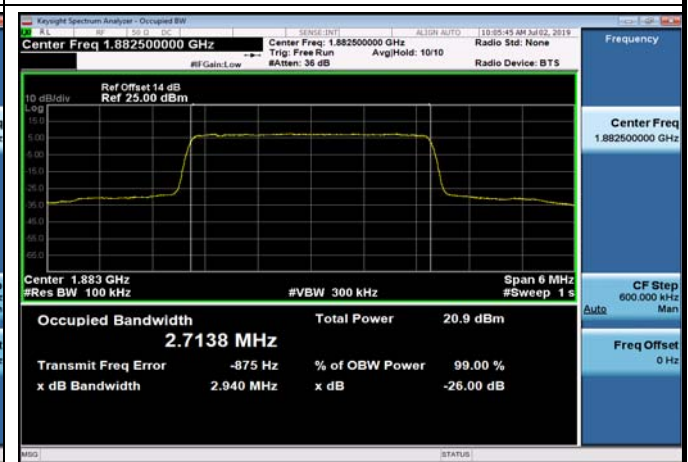
FDD25_MidRange_5_1882.5_Q16
