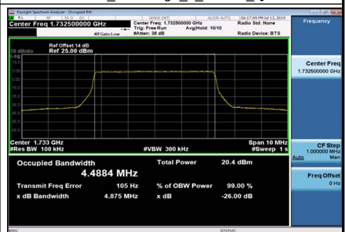
FDD04_MidRange_5_1732.5_Q16
