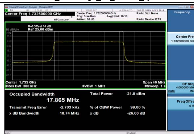
FDD04_MidRange_20_1732.5_QPSK
