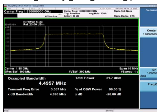
FDD02_MidRange_5MHz_1880MHz_QPSK
