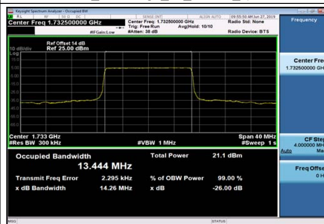
FDD04_MidRange_20_1732.5_QPSK
