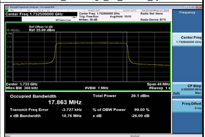
FDD04_MidRange_20_1732.5_Q16
