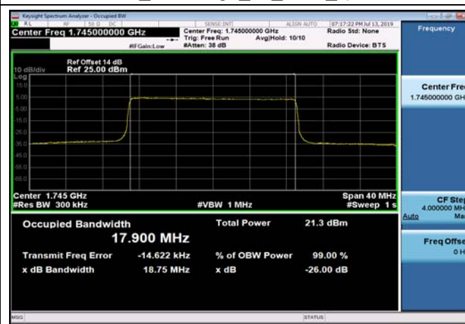
FDD66_MidRange_20_1745_QPSK
