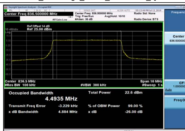
FDD05_MidRange_5MHz_836.5MHz_QPSK
