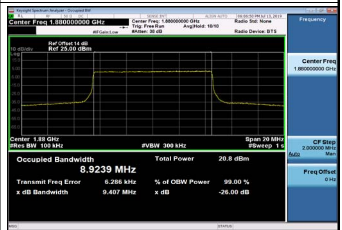
FDD02_MidRange_15_1880_Q16
