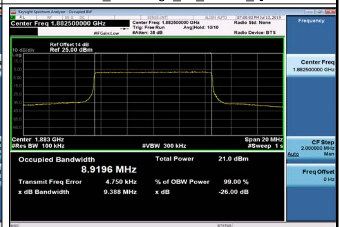
FDD25_MidRange_10_1882.5_Q16
