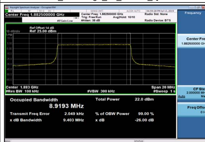
FDD25_MidRange_10_1882.5_QPSK
