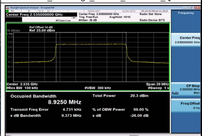
FDD07_MidRange_10MHz_2535MHz_Q16
