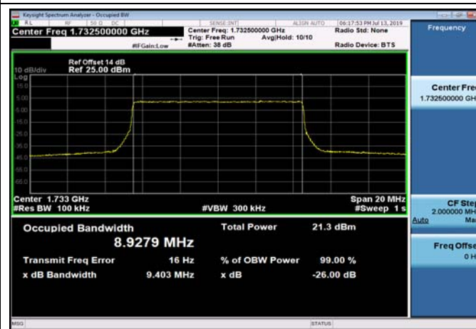
FDD04_MidRange_15_1732.5_QPSK
