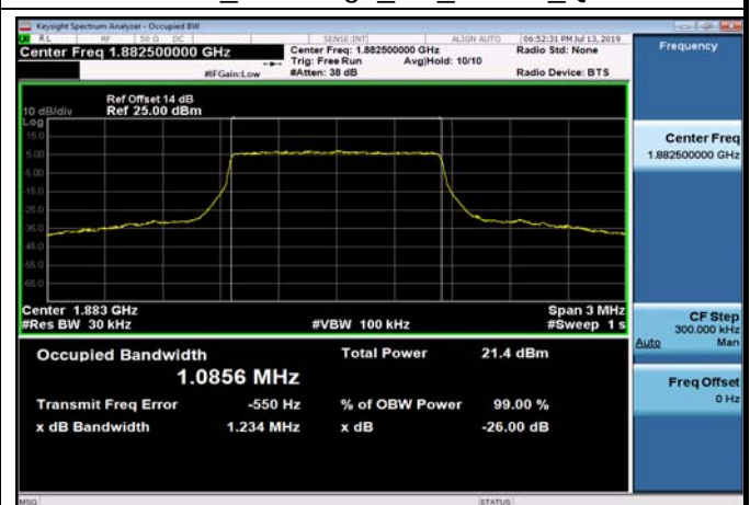
FDD25_MidRange_1.4_1882.5_Q16
