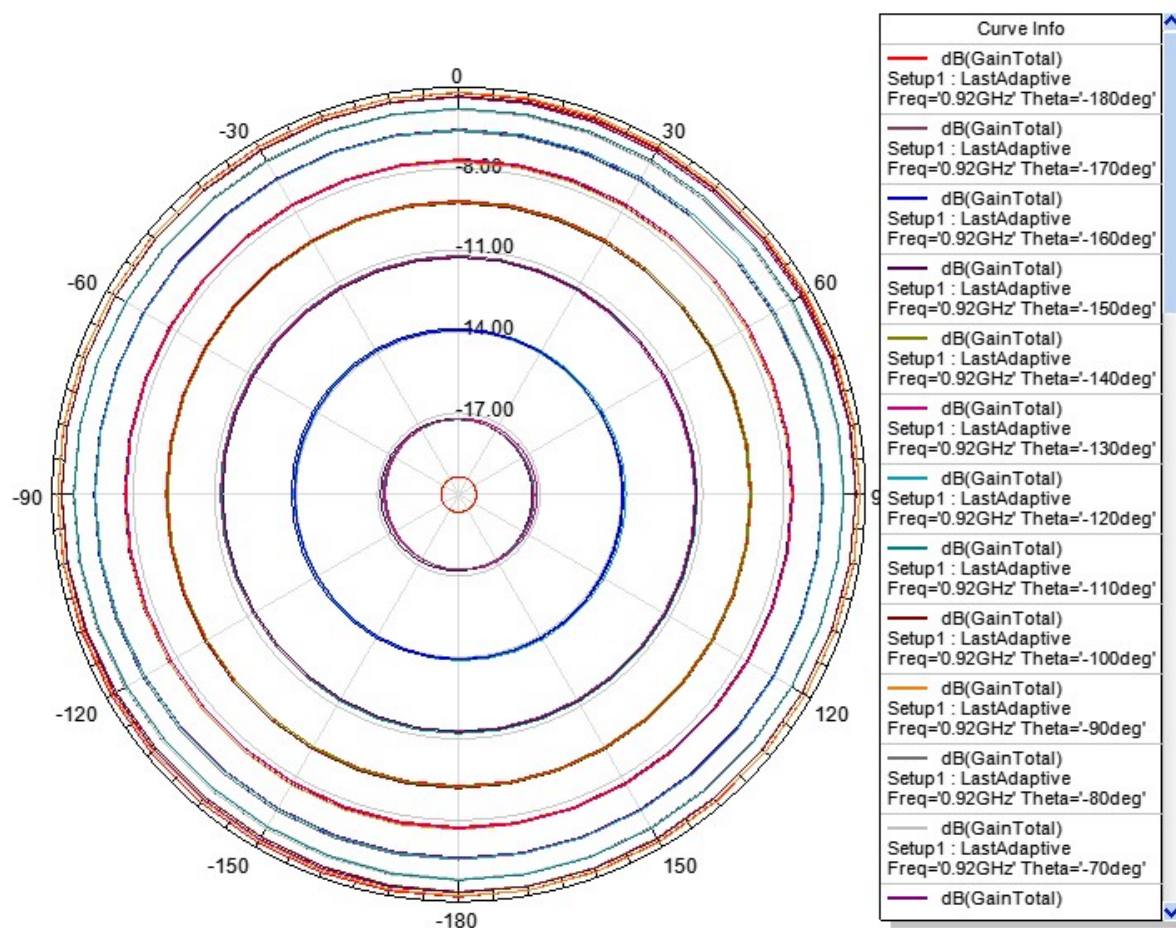
Fre=920Mhz 2D pattern
