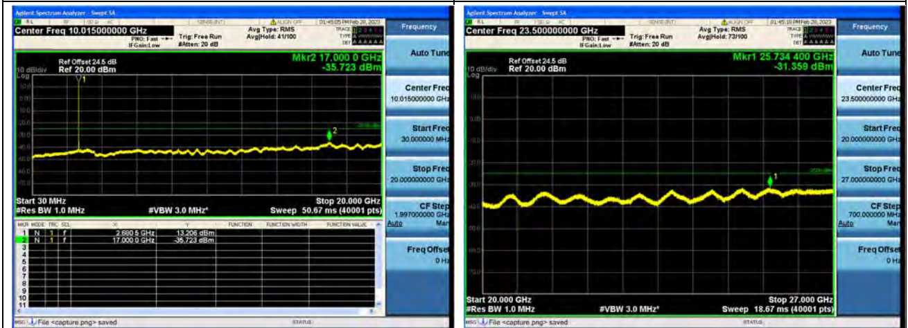
Band41-30M-20G / 10MHz / High CH / 16QAM
