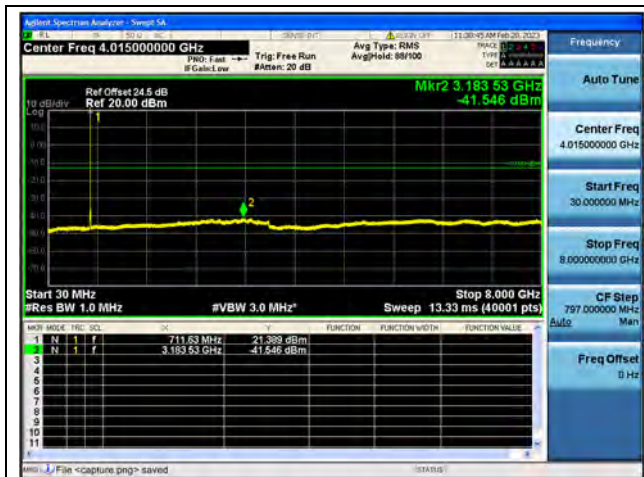
Band12 / 5MHz / High CH / QPSK
