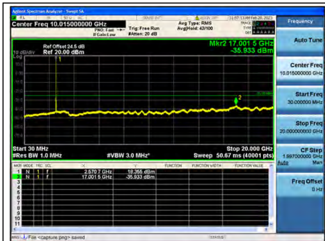
Band38-30M-20G / 20MHz / Low CH / QPSK
