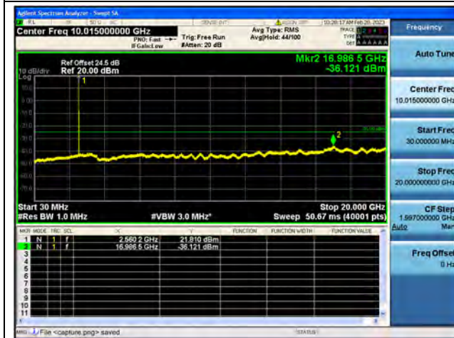
Band7-30M-20G / 10MHz / High CH / 16QAM
