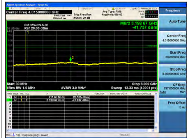
Band17 / 5MHz / High CH / 64QAM
