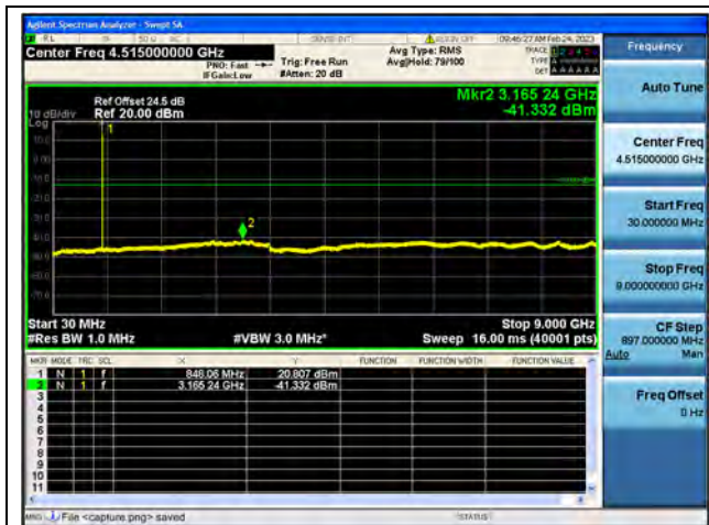
Band5 / 1.4MHz / High CH / QPSK
