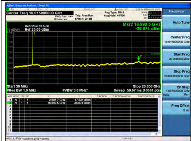
Band38-30M-20G / 20MHz / Mid CH / 16QAM
