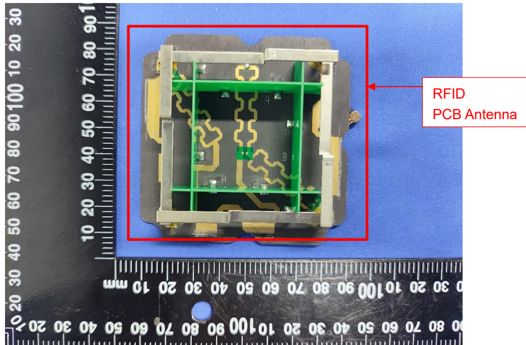
SECONDARY BOARD 6 TOP VIEW
