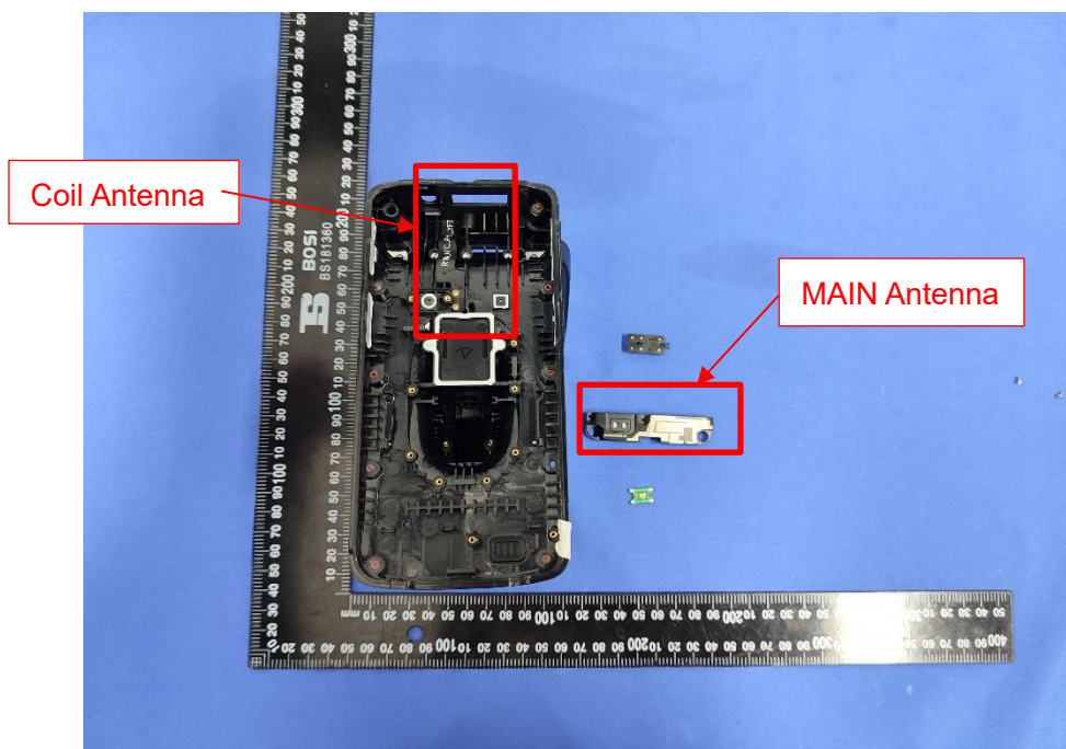
EUT UNCOVER VIEW 4
