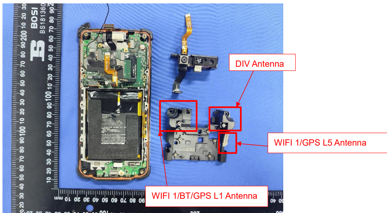
EUT UNCOVER VIEW 7
