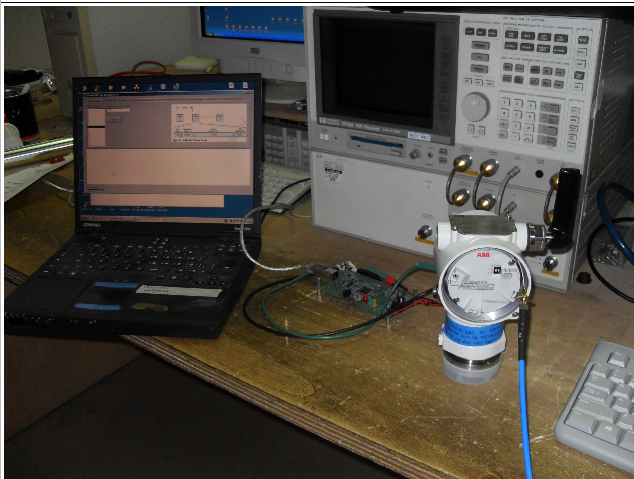
Antenna Port Conducted Emissions Test Set-up
