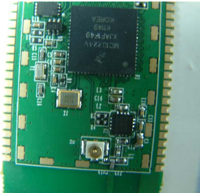
Oscillator view
