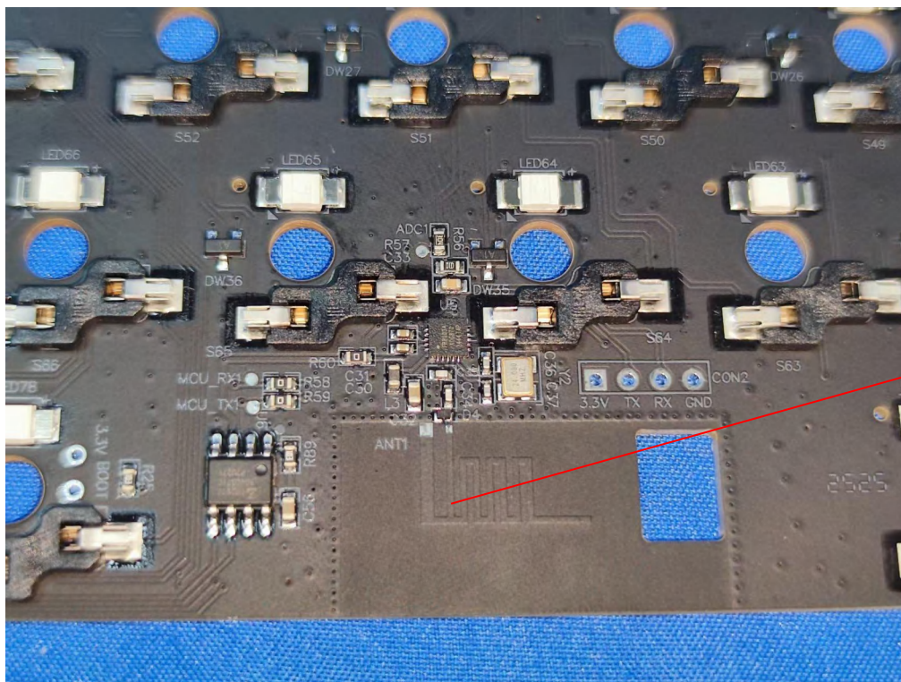
Integral Antenna
