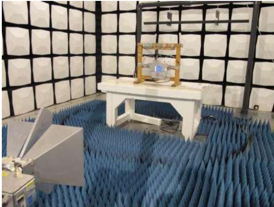
Radiated emission 1 – 18 GHz
