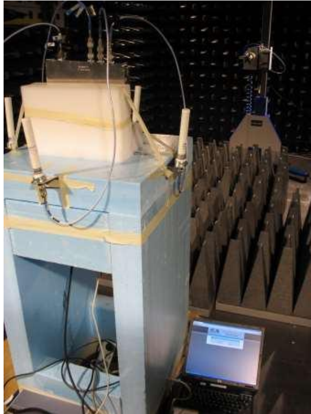
Radiated emission 18-26 GHz preliminary sweep
