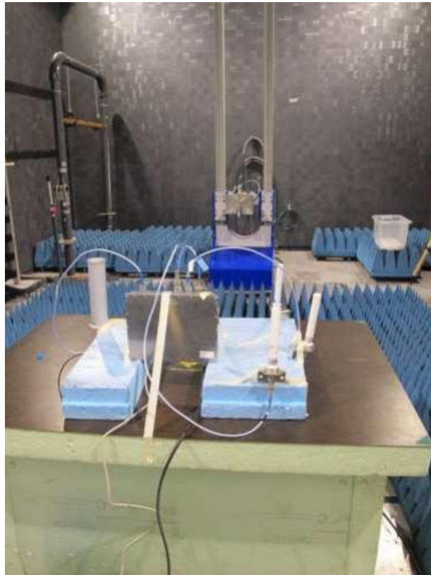
Radiated emission 30 MHz – 1 GHz
