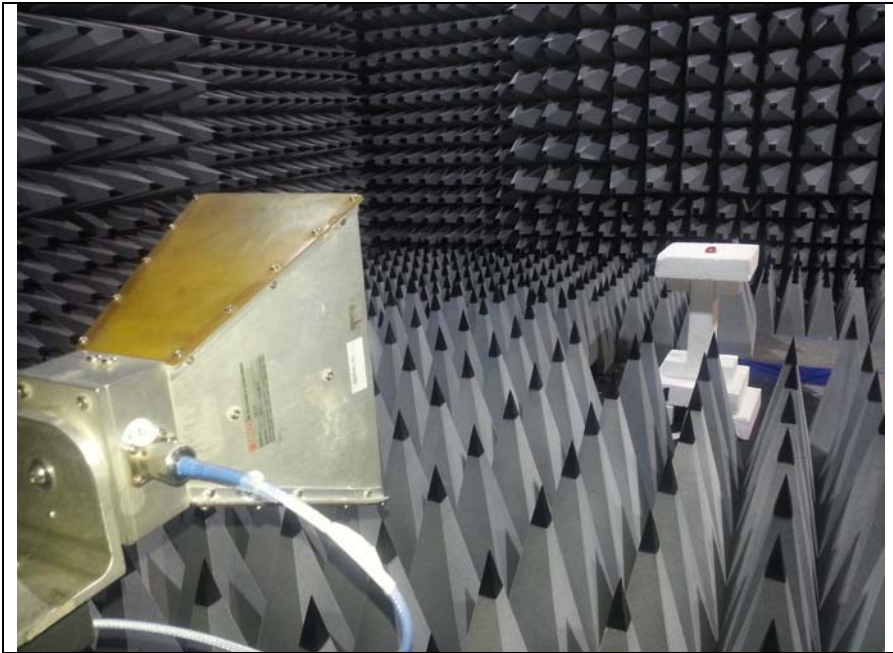
Fig 3 Test setup 1GHz -18GHz Rad Emissions
