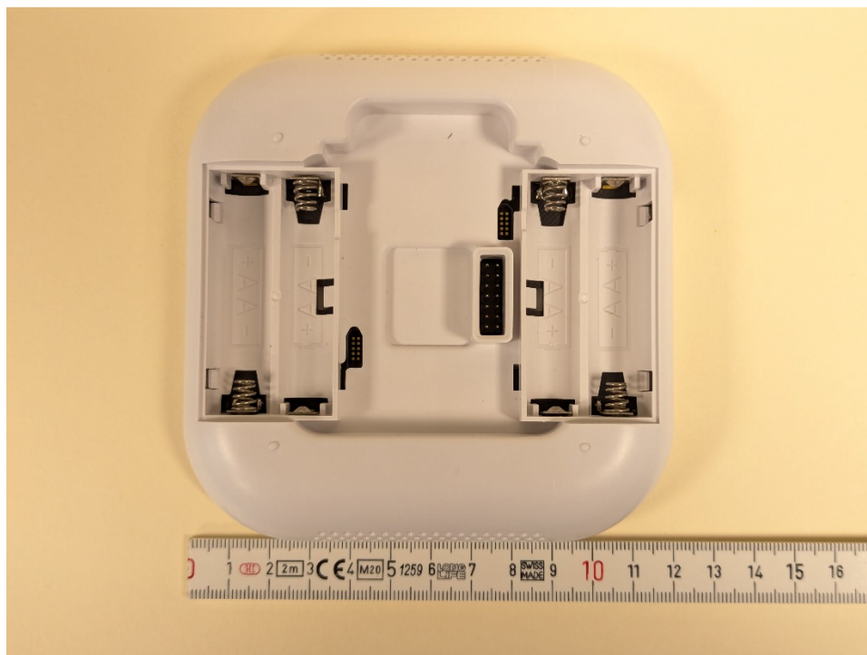
Bottom / Back – Battery Cover Removed
