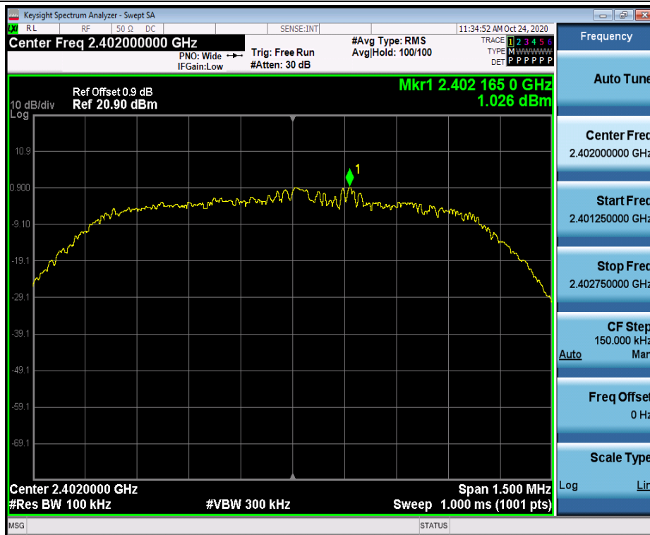
2DH5_Ant1_2402_0~Reference
