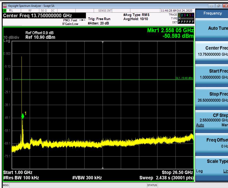
3DH5_Ant1_2441_0~Reference
