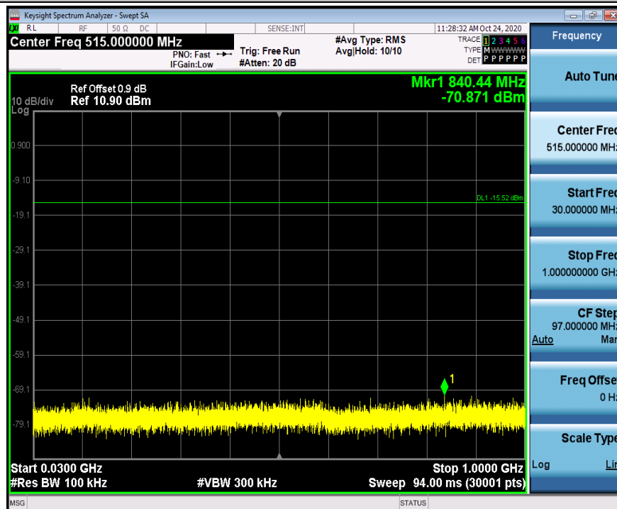
DH5_Ant1_2402_30~1000
