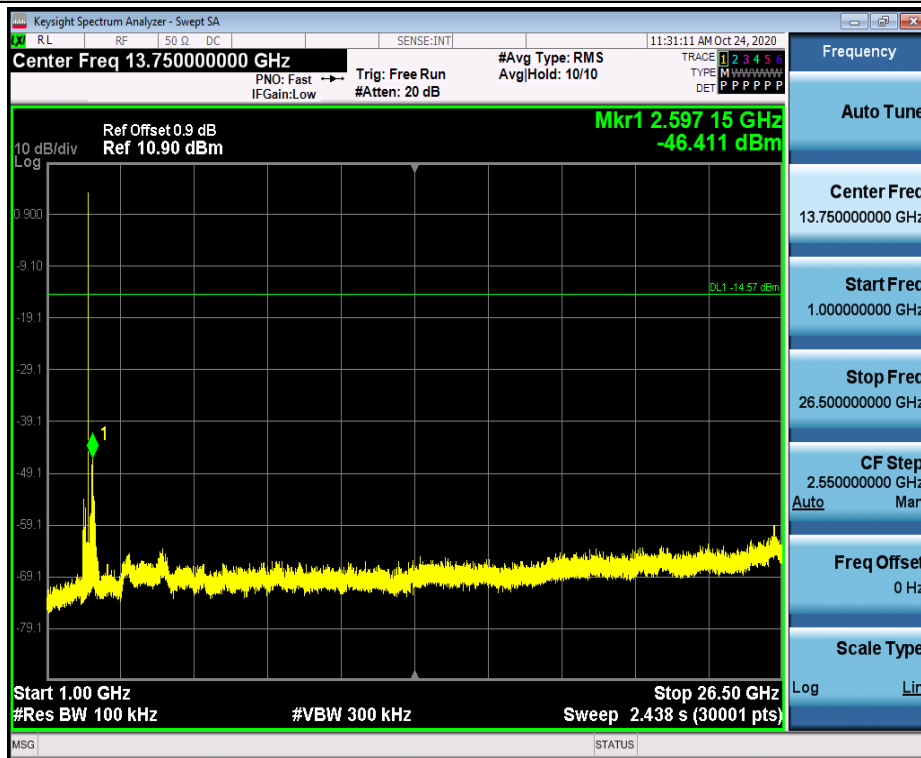
DH5_Ant1_2441_1000~26500
