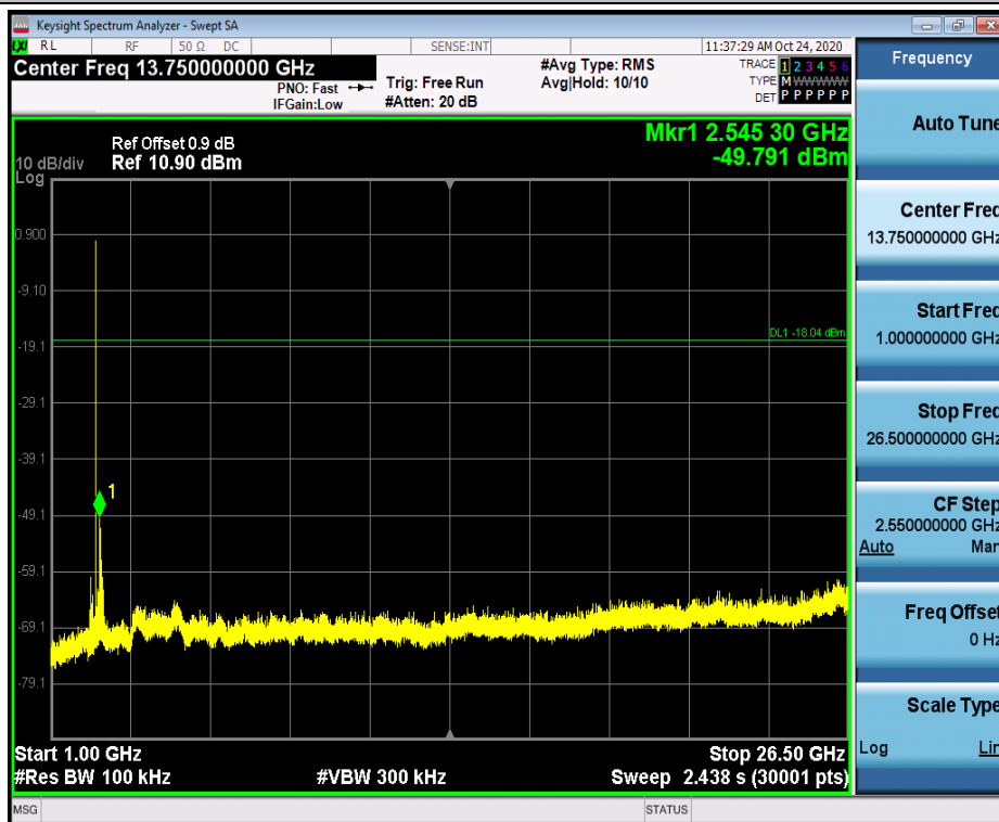
2DH5_Ant1_2480_0~Reference
