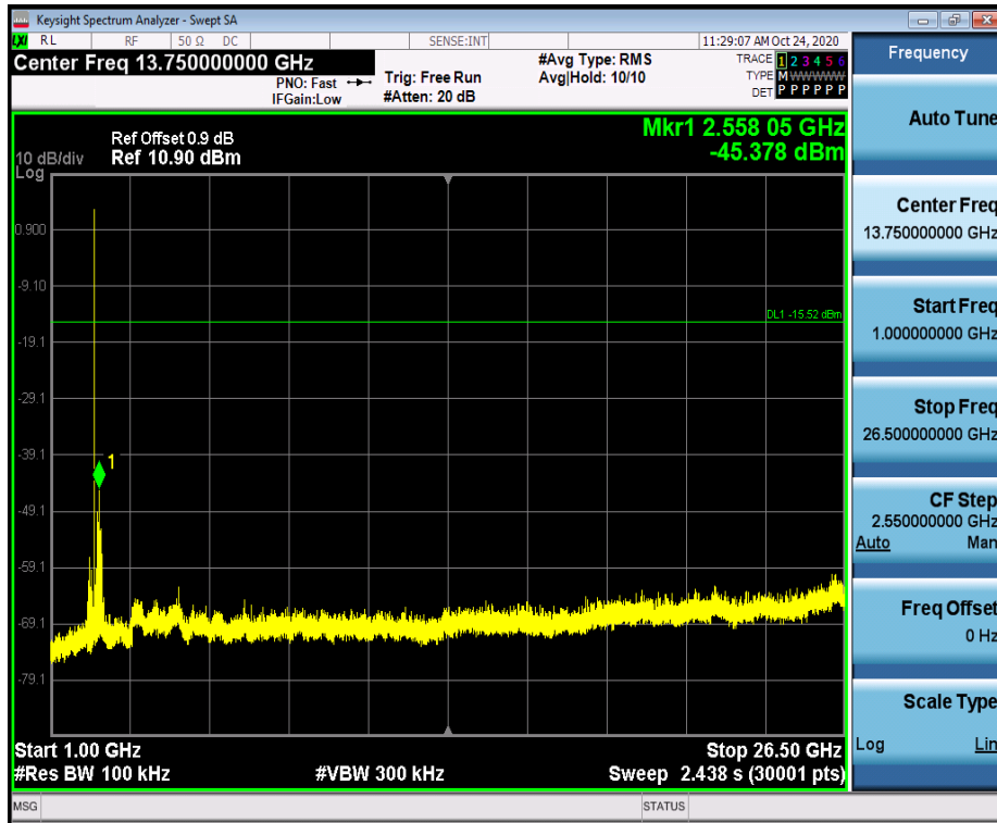
DH5_Ant1_2441_0~Reference
