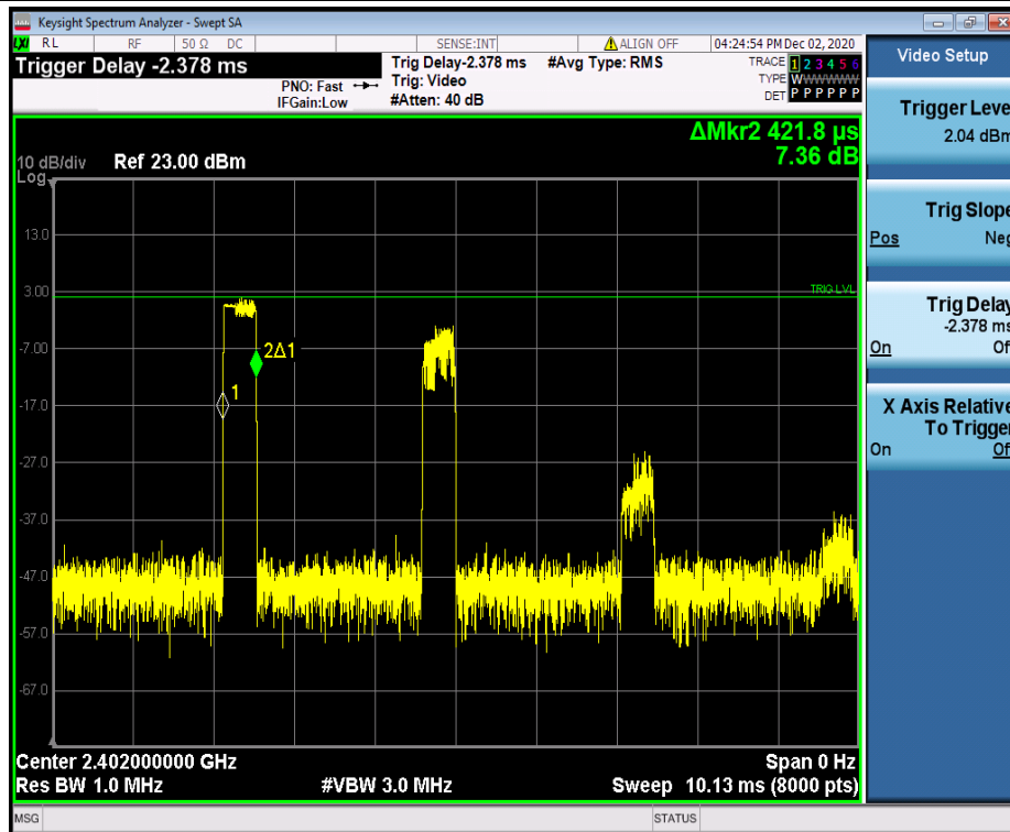
3DH1_Ant1_Hop_2402
