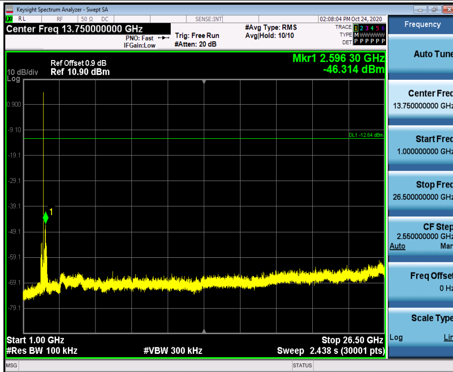
BLE_1M_Ant1_2440_1000~26500
