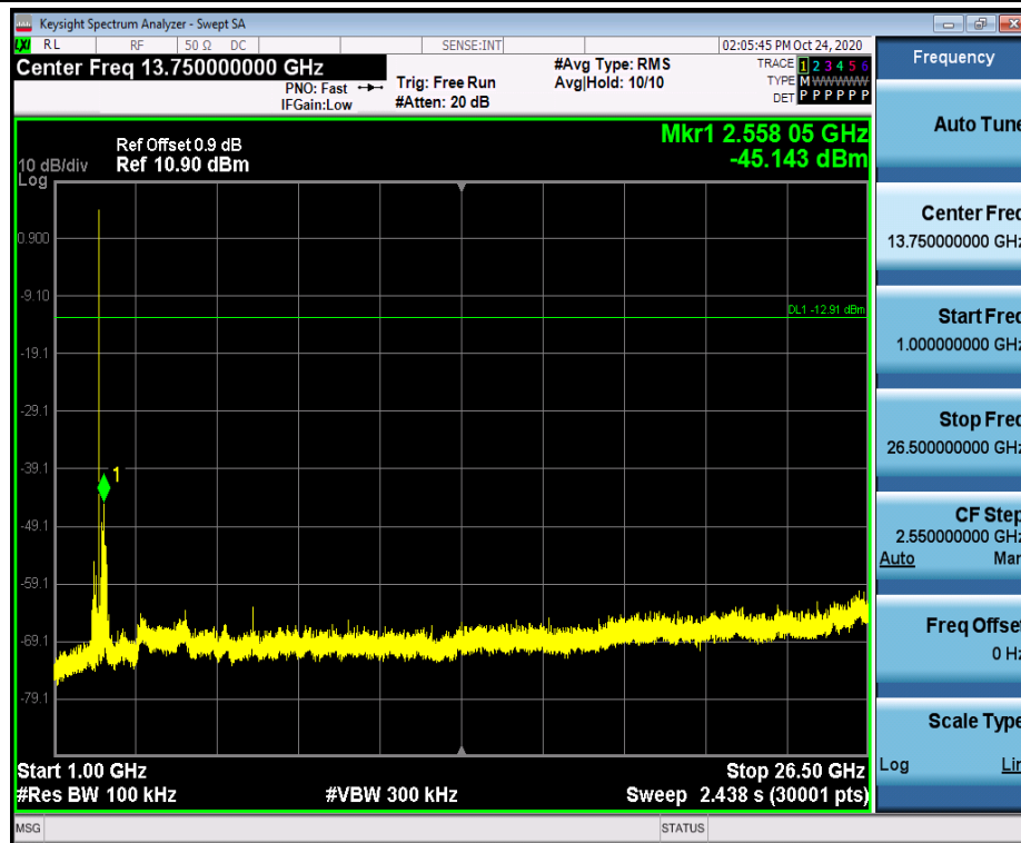
BLE_1M_Ant1_2440_0~Reference
