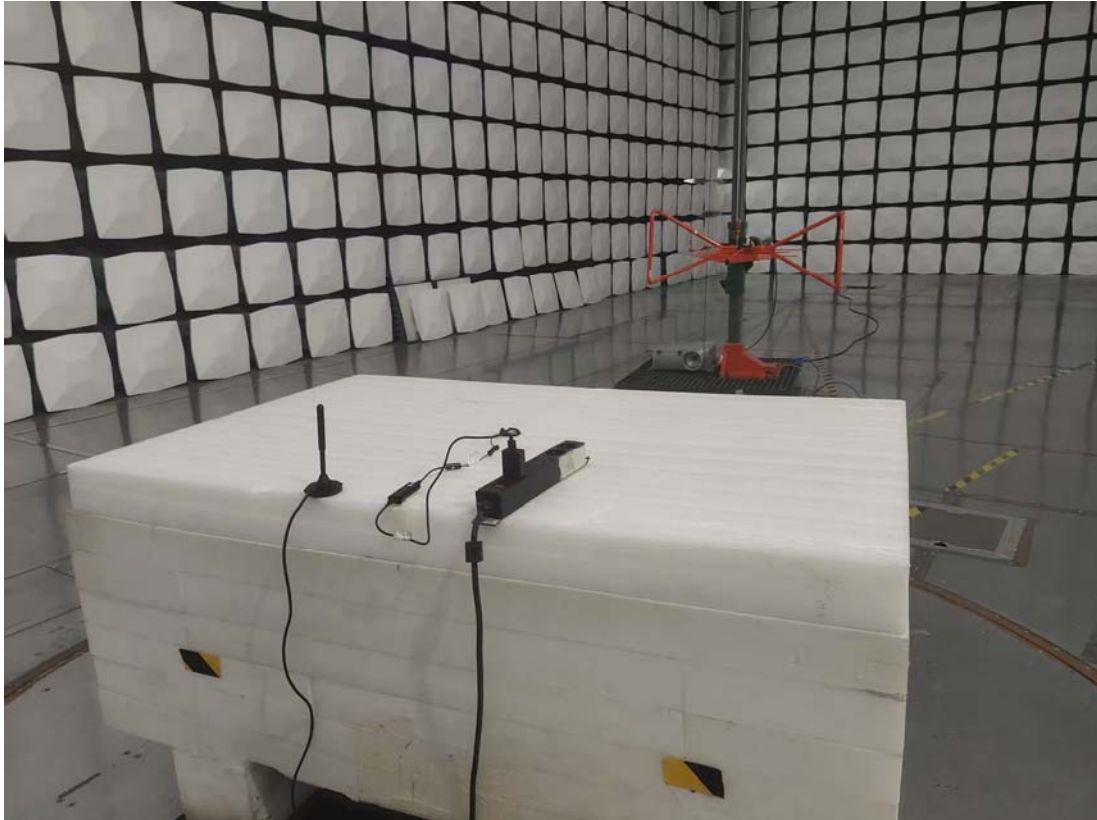
Radiated Emissions Below 1G side View
