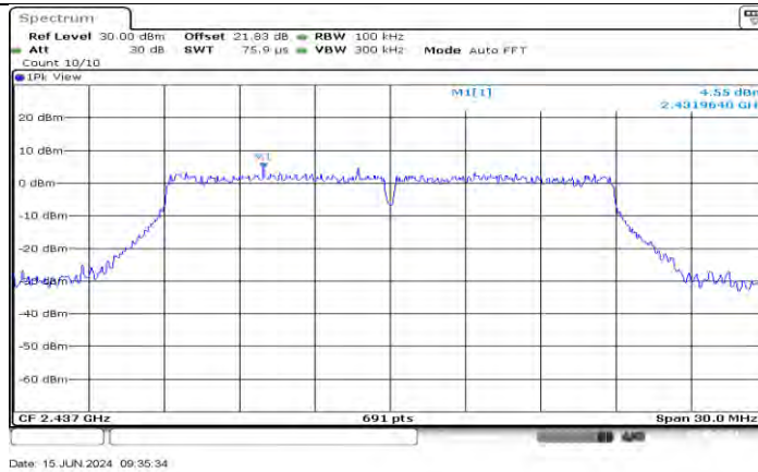
11N20SISO_Ant1_2437_0~Reference
