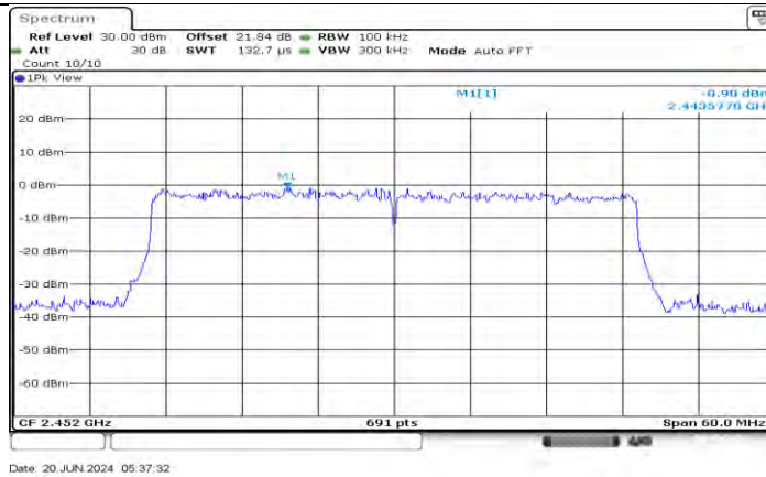
11AX40SISO_Ant1_2452_0~Reference
