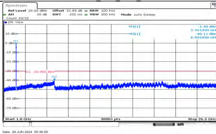
11AX40SISO_Ant1_2452_1000~26500
