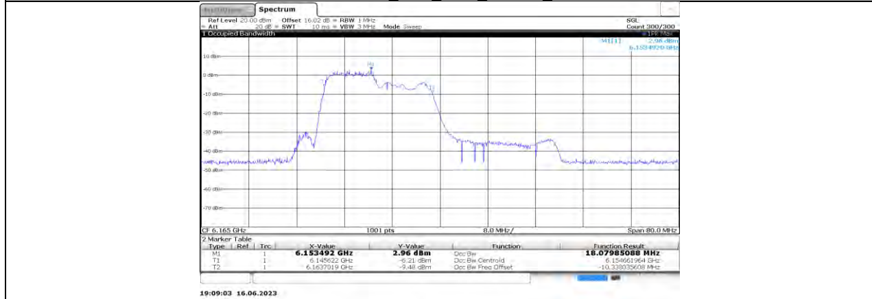
11AX40MIMO Ant0_6165_106Tone_RU53
