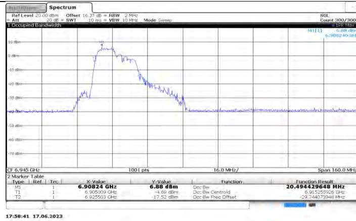
11AX80MIMO Ant0 6945 106Tone RU53
