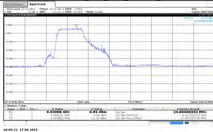
11AX80MIMO Ant0 6945 242Tone RU61
