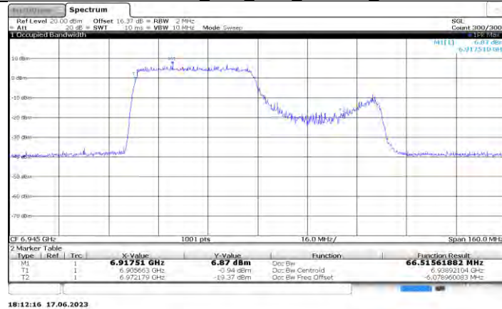
11AX80MIMO Ant0 6945 484Tone RU65
