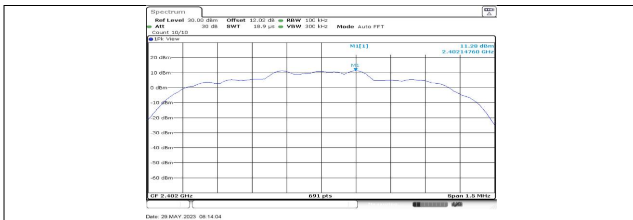
3DH5_Ant1_2402_0~Reference
