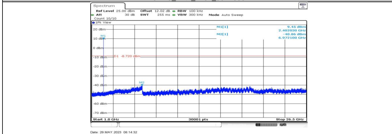
3DH5_Ant1_2402_1000~26500
