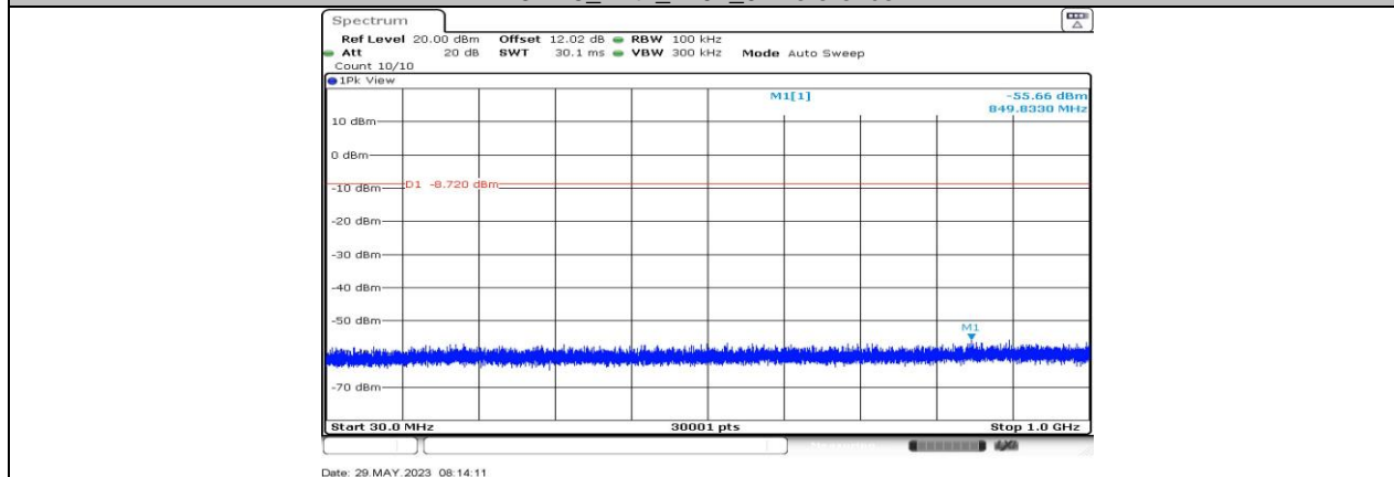
3DH5_Ant1_2402_30~1000
