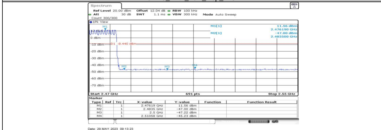
3DH5_Ant1_High_Hop_2480
