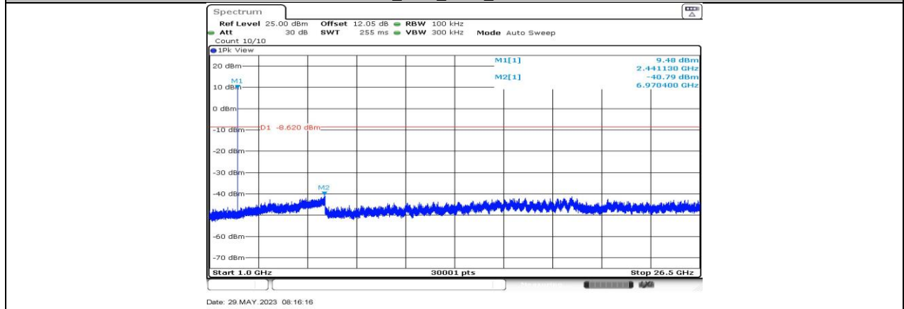
3DH5_Ant1_2441_1000~26500
