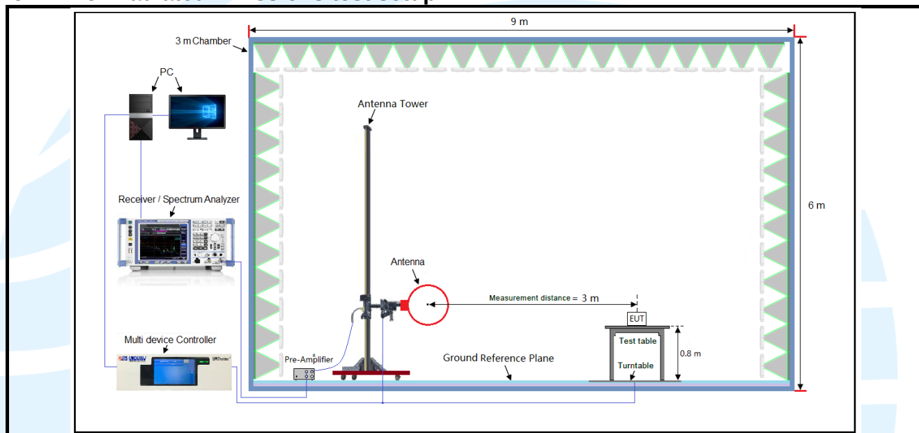
Figure 1. Below 30MHz
