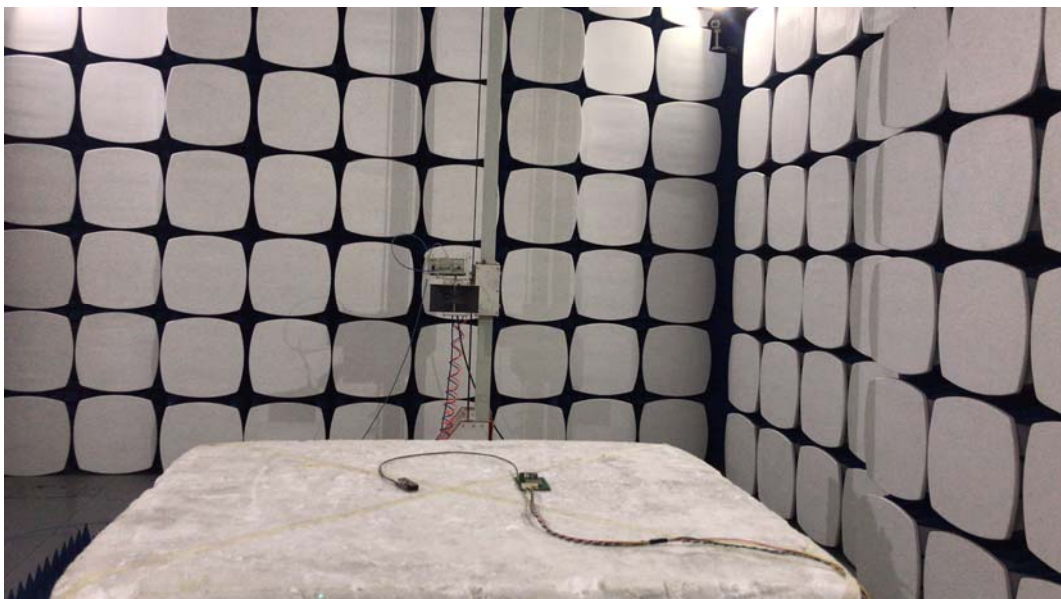
Radiated Emission Above 1G Test Photo
