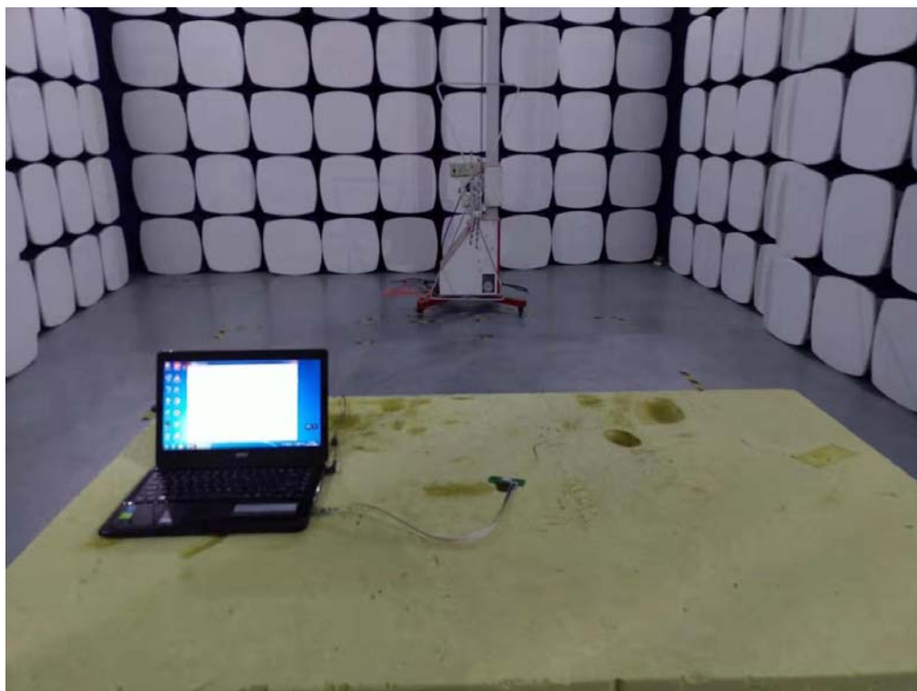
Radiated Emission Above 1G Test Photo
