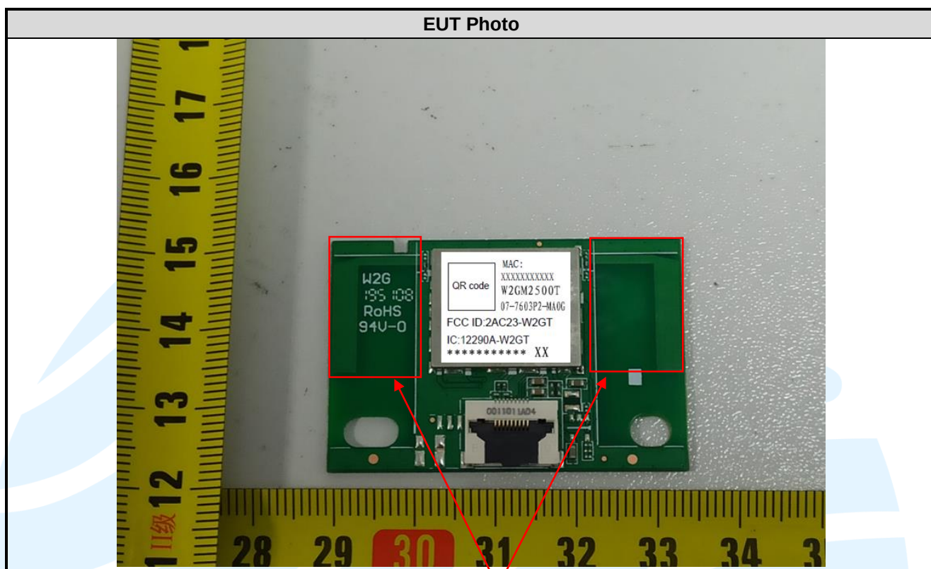
WiFi Antenna
