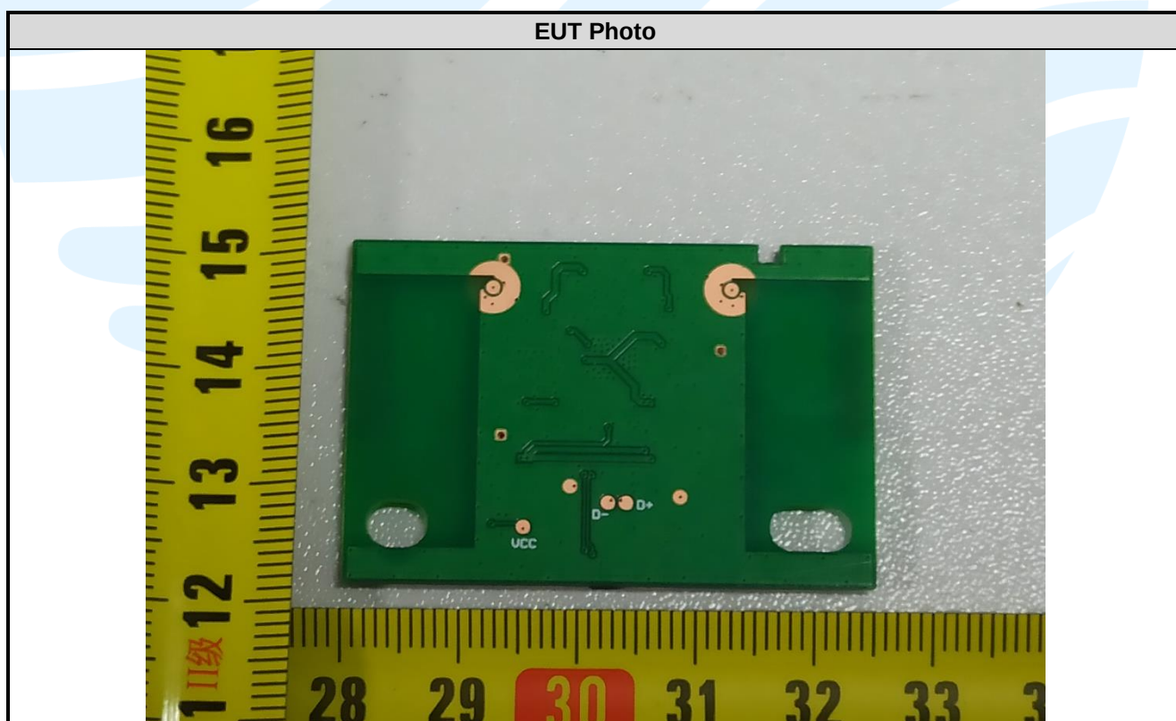
WiFi Antenna
