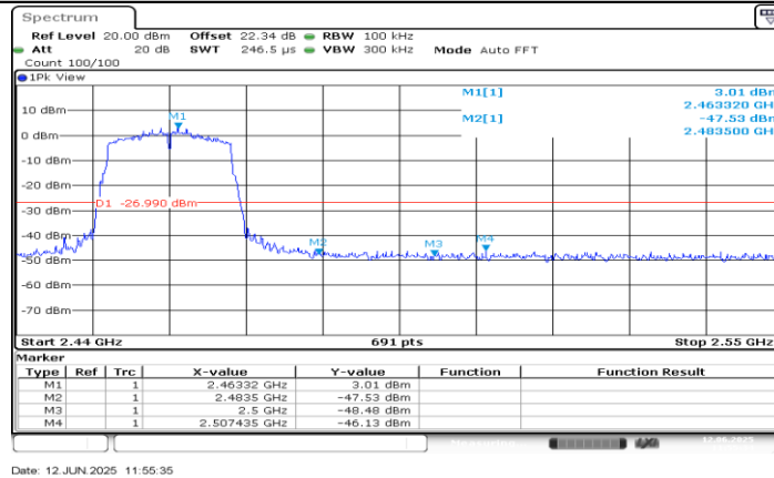
11N20SISO_Ant0_High_2462
