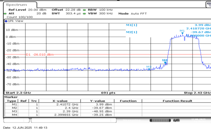
11N20SISO_Ant0_Low_2412
