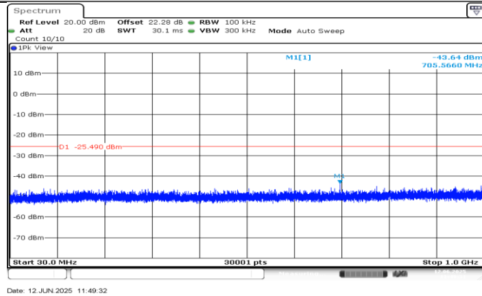
11N20SISO_Ant0_2412_30~1000
