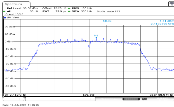
11N20SISO_Ant0_2412_0~Reference
