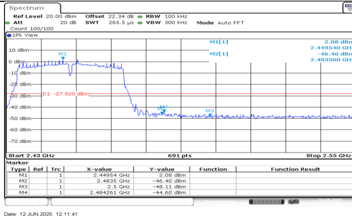
11N40SISO_Ant0_High_2452
