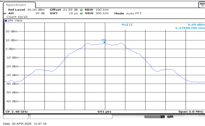
BLE_1M_Ant BT_2480_0-Reference
