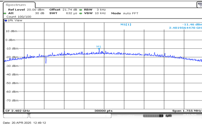
BLE_2M_Ant BT_2402
