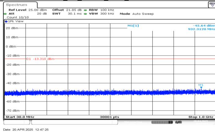
BLE_1M_Ant BT_2480_30-1000
