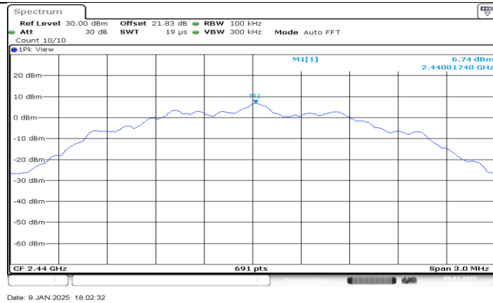
BLE_2M_Ant BT_2440_0-Reference
