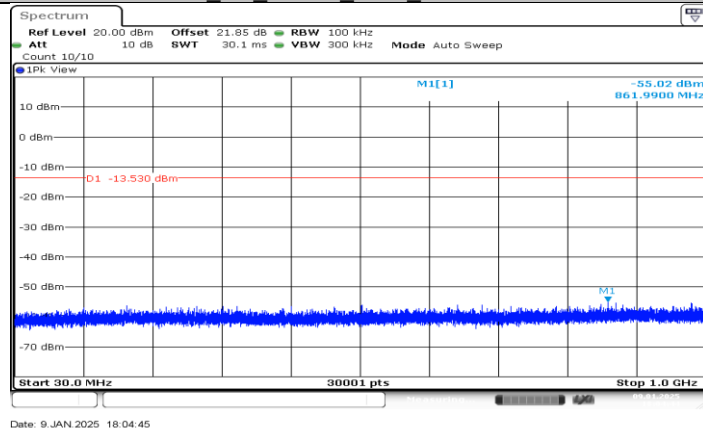
BLE_2M_Ant BT_2480_30-1000
