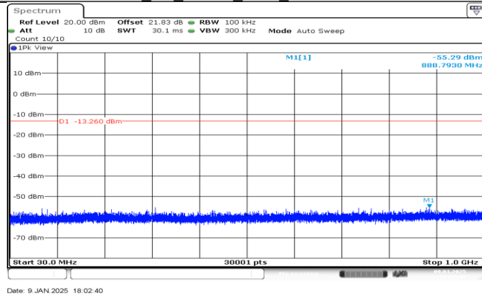
BLE_2M_Ant BT_2440_30-1000
