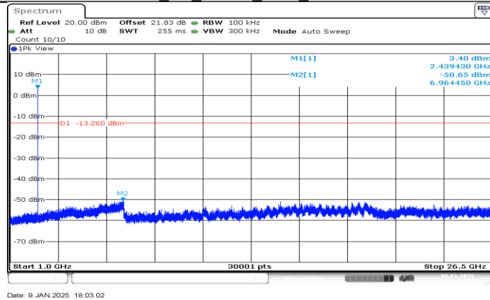
BLE_2M_Ant BT_2440_1000-26500
