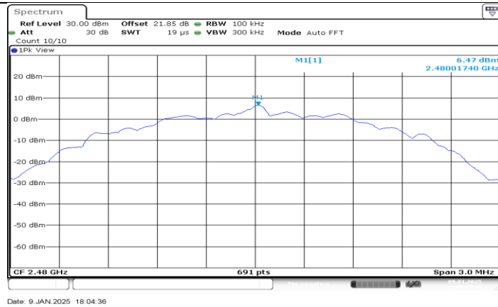
BLE_2M_Ant BT_2480_0-Reference
