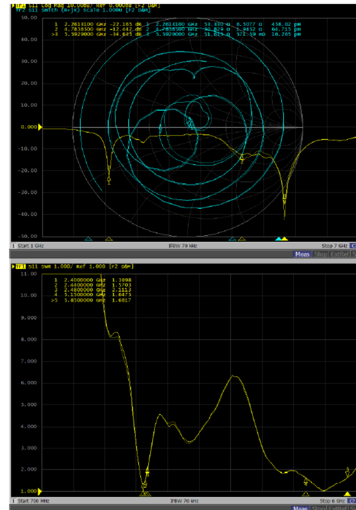
WIFI 1-2.4G-5G
