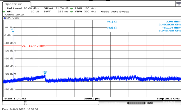
3DH5_Ant BT_2402_1000~26500
