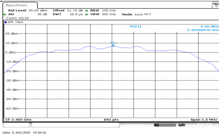
3DH5_Ant BT_2402_0~Reference
