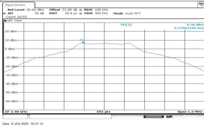
DH5_Ant BT_2480_0~Reference
