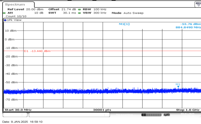
3DH5_Ant BT_2402_30~1000
