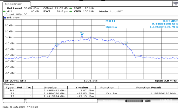
3DH5_Ant BT_2441
