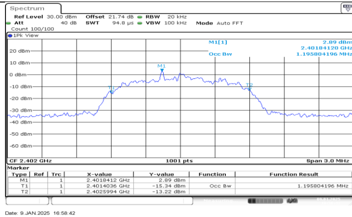
3DH5_Ant BT_2402
