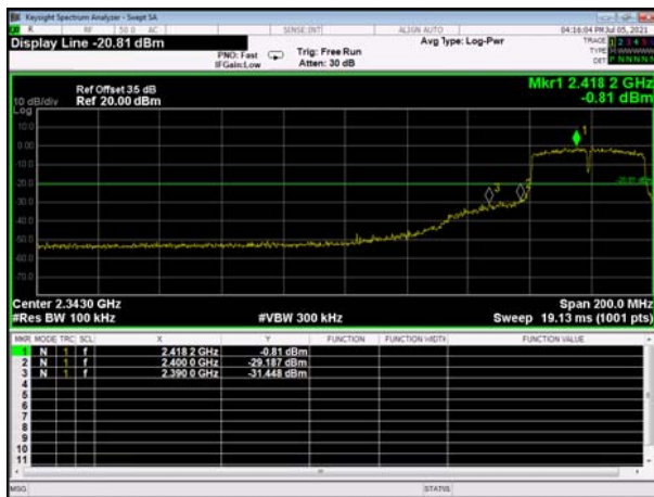
Bandedge-CH03
