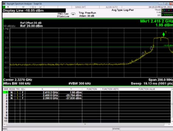
Bandedge-CH01
