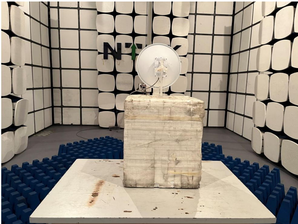
Radiated Measurement Photos 18GHz~40GHz (25dBi Antenna)
