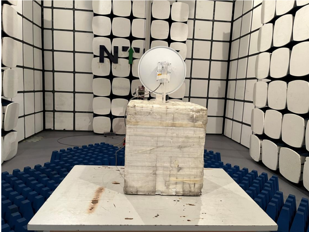
Radiated Measurement Photos 1GHz~18GHz (25dBi Antenna)
