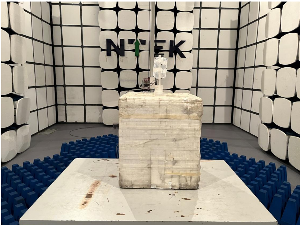
Radiated Measurement Photos 1GHz~18GHz (8dBi Antenna)
