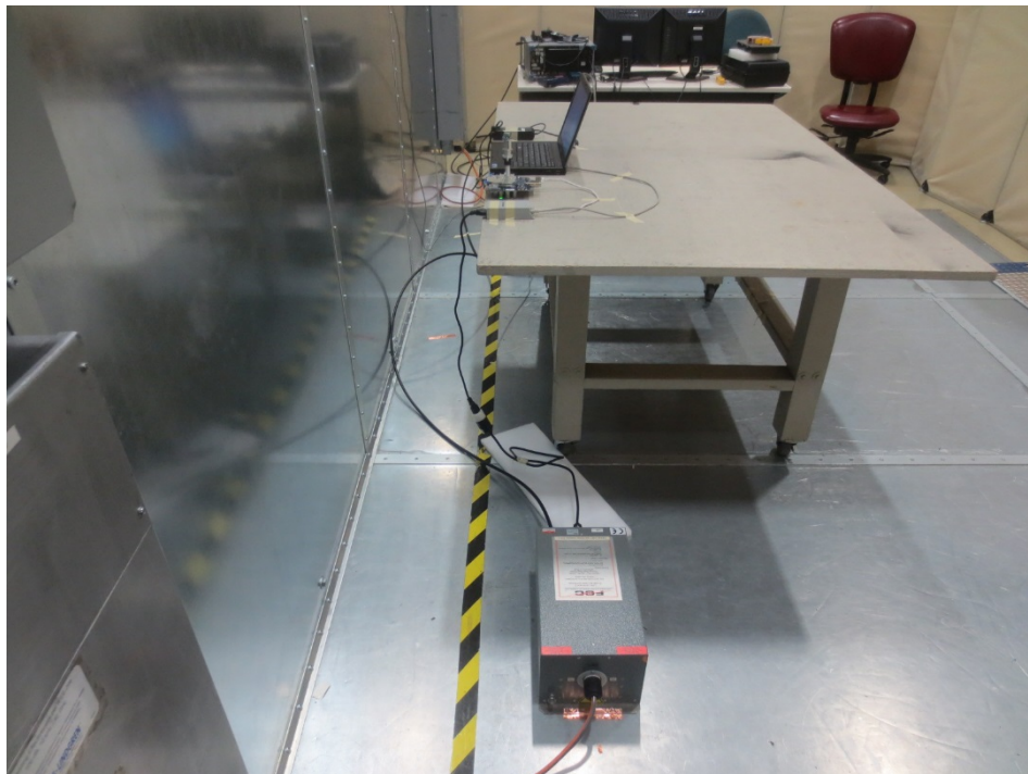
1.16 AC Line Conducted Emissions Left Side View
