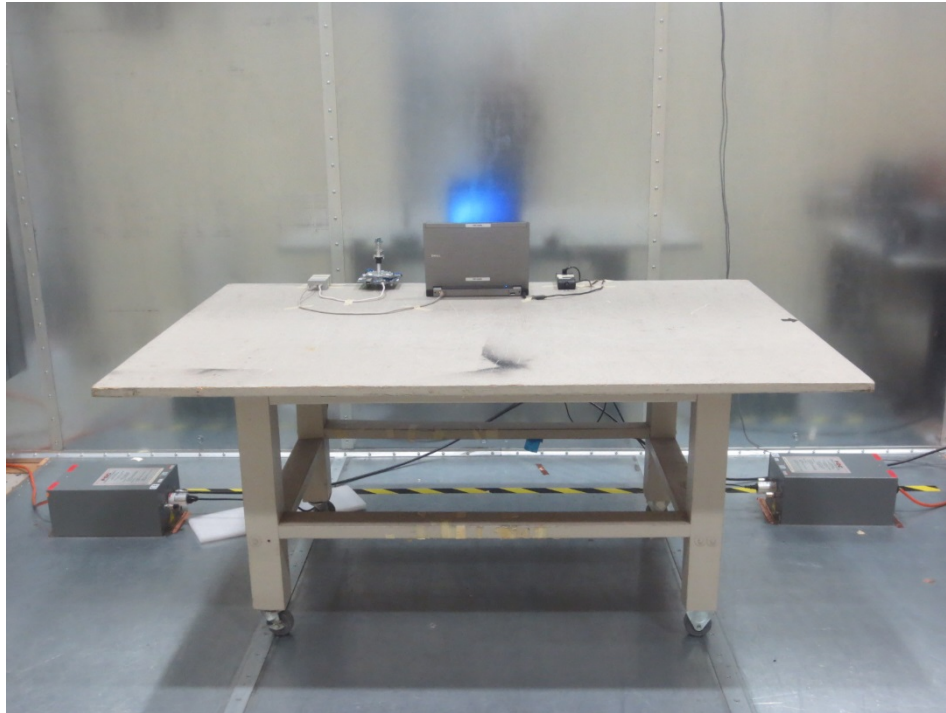
1.15 AC Line Conducted Emissions Front View
