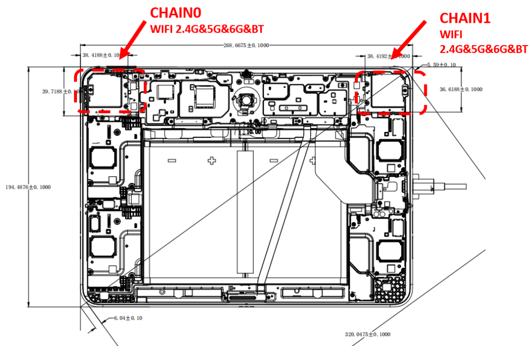
Picture 10 Antenna location
