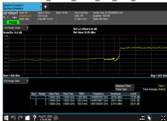
N25(40M)_DFT-s- OFDM_BPSK_Outer_Full_Low_CH
