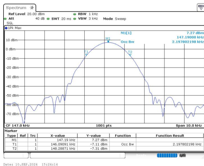
99% Occupied Bandwidth Plot
