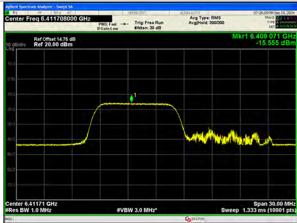
PSD NVNT be20 106@53 6415MHz Ant13 MIMO
