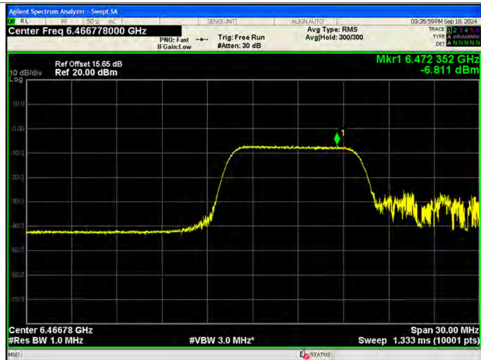
PSD NVNT be20 106@53 6475MHz Ant12 SISO
