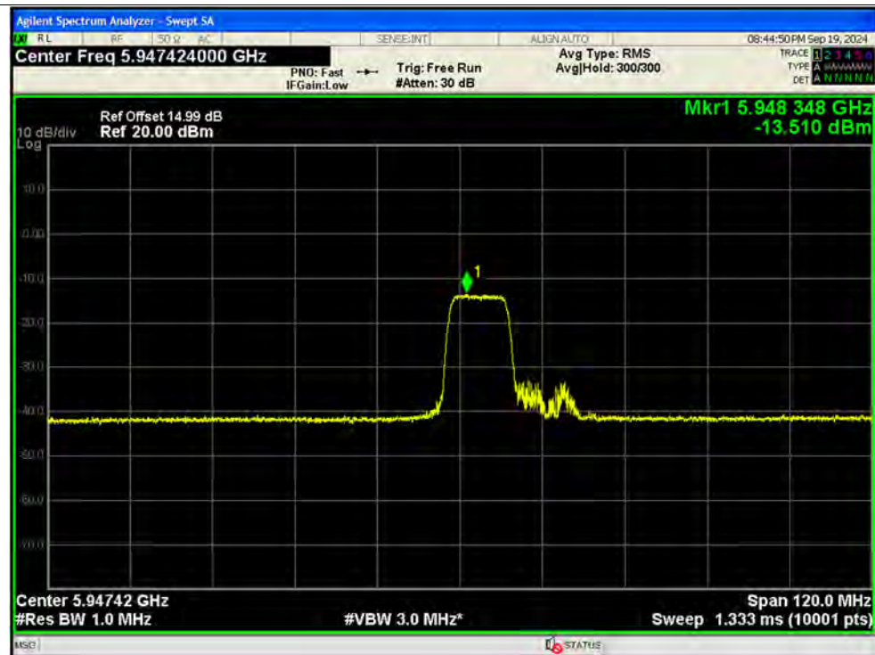
PSD NVNT be80 106@53 5985MHz Ant13 MIMO
