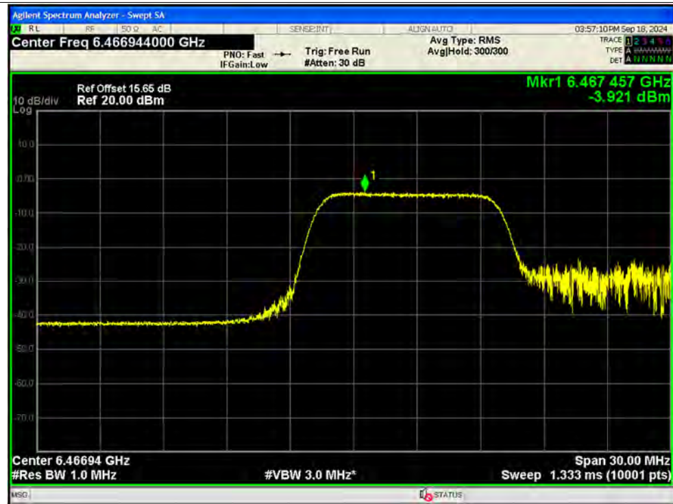
PSD NVNT be20 106@53 6475MHz Ant13 MIMO
