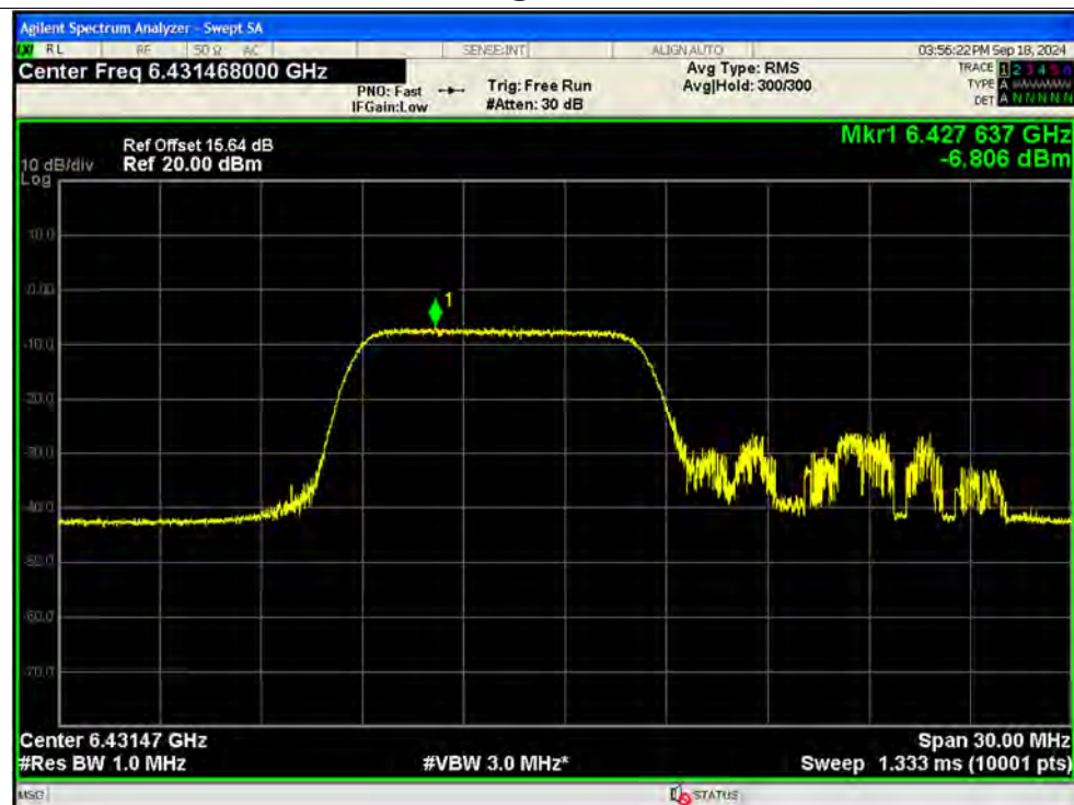
PSD NVNT be20 106@53 6435MHz Ant13 MIMO
