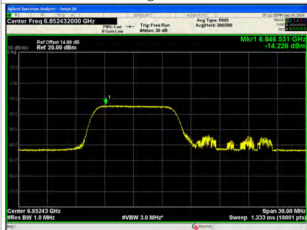
PSD NVNT be20 106@53 6855MHz Ant12 SISO
