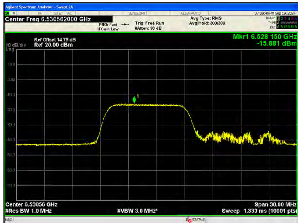
PSD NVNT be20 106@53 6535MHz Ant12 SISO
