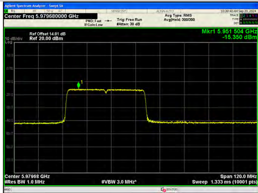
PSD NVNT be80 484@65 5985MHz Ant13 MIMO
