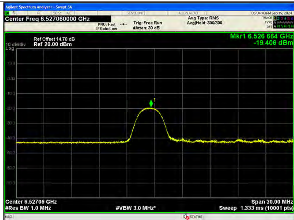
PSD NVNT be20 26@0 6535MHz Ant13 MIMO
