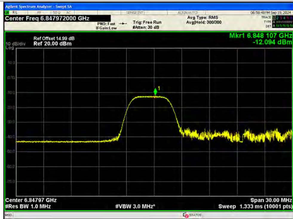
PSD NVNT be20 52@37 6855MHz Ant13 MIMO
