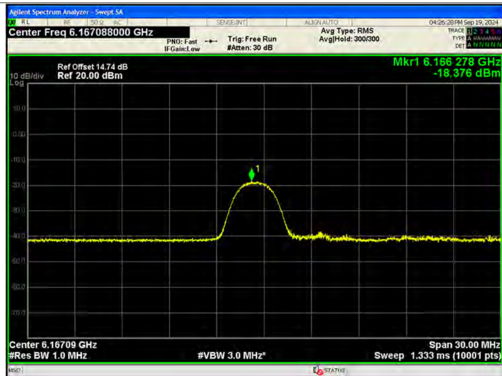
PSD NVNT be20 26@0 6175MHz Ant13 MIMO
