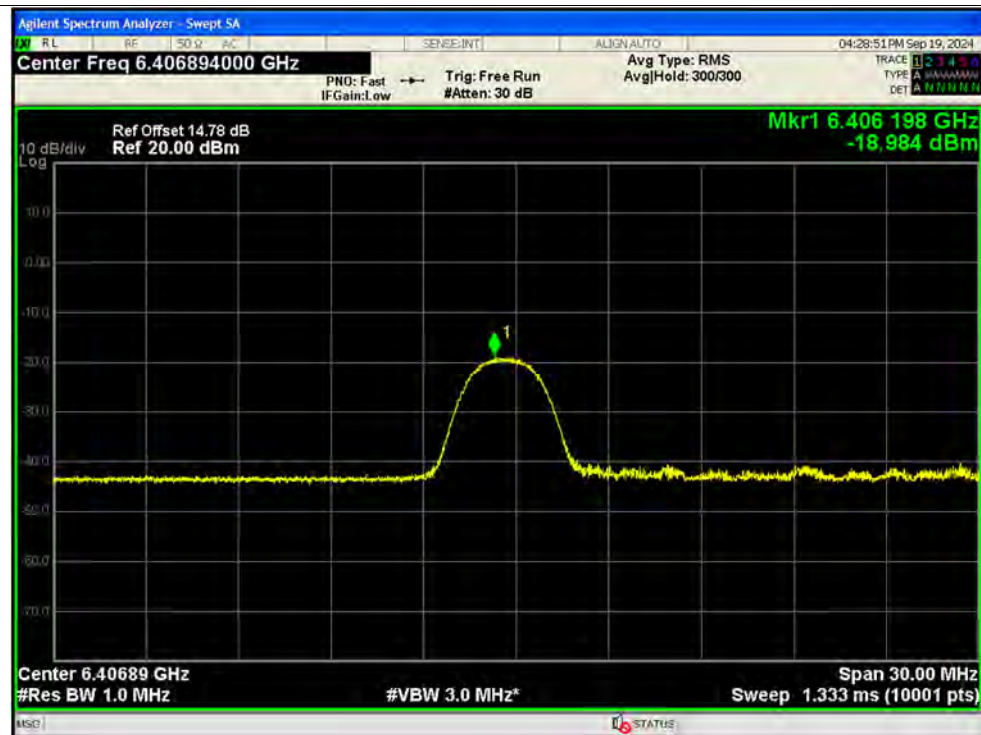
PSD NVNT be20 26@0 6415MHz Ant13 MIMO
