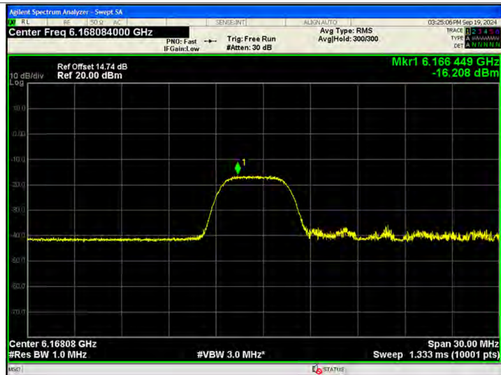
PSD NVNT ax20 52@37 6175MHz Ant13 SISO
