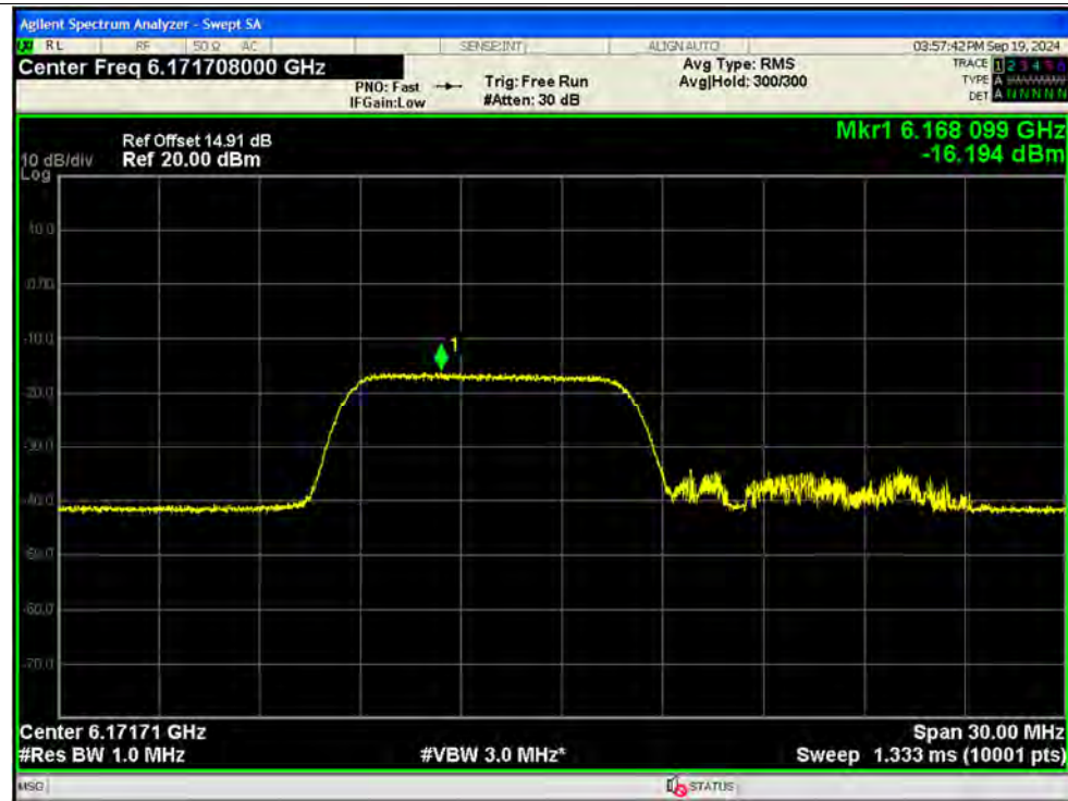
PSD NVNT ax20 106@53 6175MHz Ant13 MIMO
