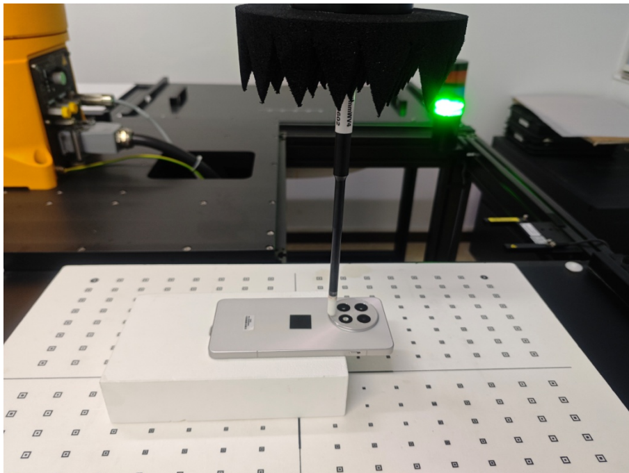
Back Side from the antenna to probe tip (Test distance: 5mm)
