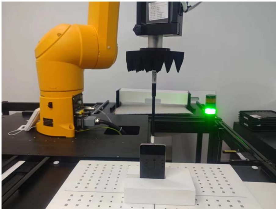
Bottom Side (Test distance: 2mm)
