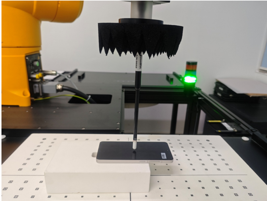
Front Side (Test distance: 2mm)
