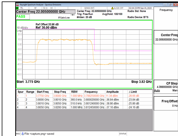
n78(3700-3800MHz) 20M DFT-s-OFDM BPSK Outer_Full High
