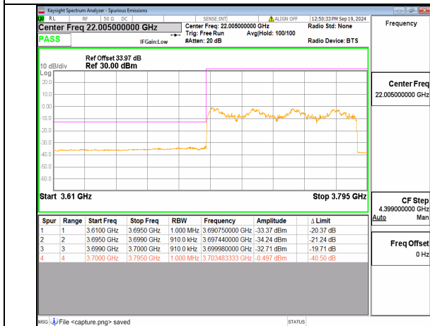
n77(3700-3980MHz) 90M DFT-s-OFDM BPSK Outer_Full Low
