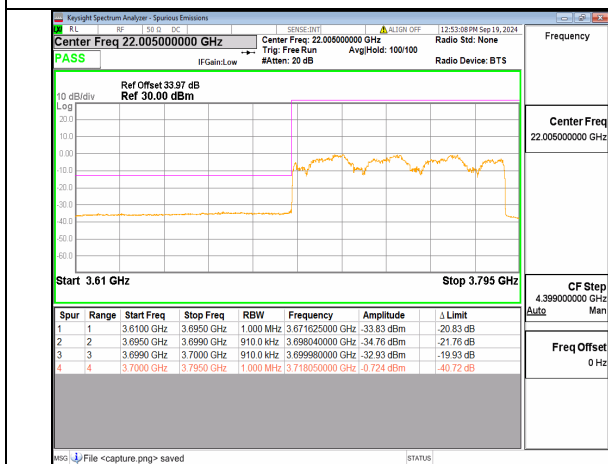
n77(3700-3980MHz) 90M DFT-s-OFDM QPSK Outer_Full Low
