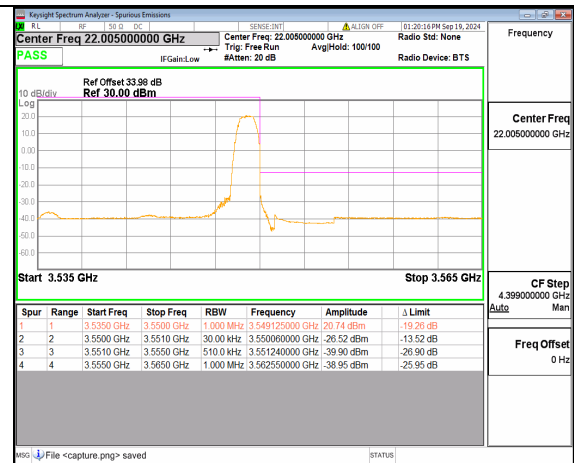
n78(3450-3550MHz) 15M DFT-s-OFDM QPSK Edge_1RB_Right High
