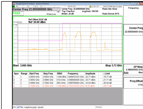
n78(3700-3800MHz) 15M DFT-s-OFDM BPSK Outer_Full Low
