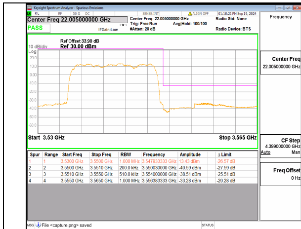
n78(3450-3550MHz) 15M DFT-s-OFDM BPSK Outer_Full High
