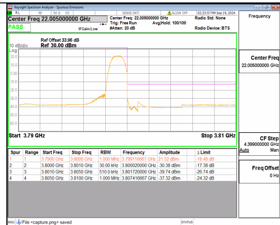
n78(3700-3800MHz) 10M DFT-s-OFDM BPSK Edge_1RB_Right High
