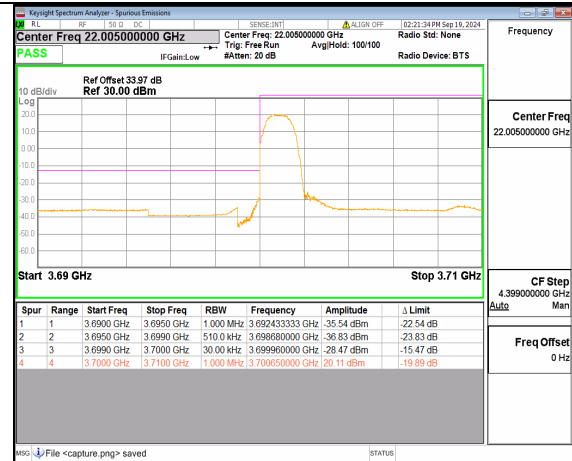
n78(3700-3800MHz) 10M DFT-s-OFDM QPSK Edge_1RB_Left Low
