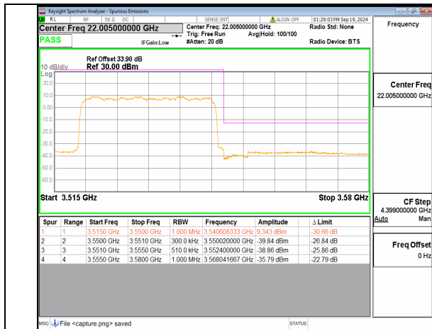
n78(3450-3550MHz) 30M DFT-s-OFDM QPSK Outer_Full High
