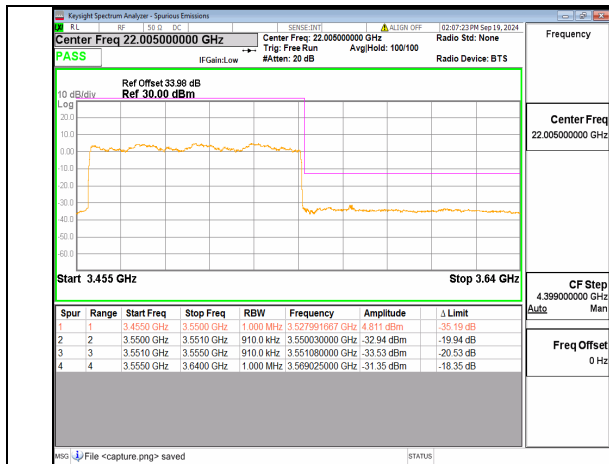
n78(3450-3550MHz) 90M DFT-s-OFDM QPSK Outer_Full High
