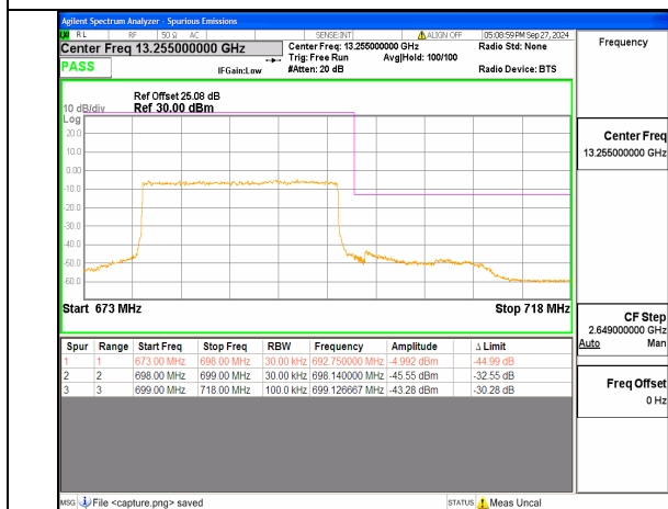
n71 20M DFT-s-OFDM BPSK Outer_Full High
