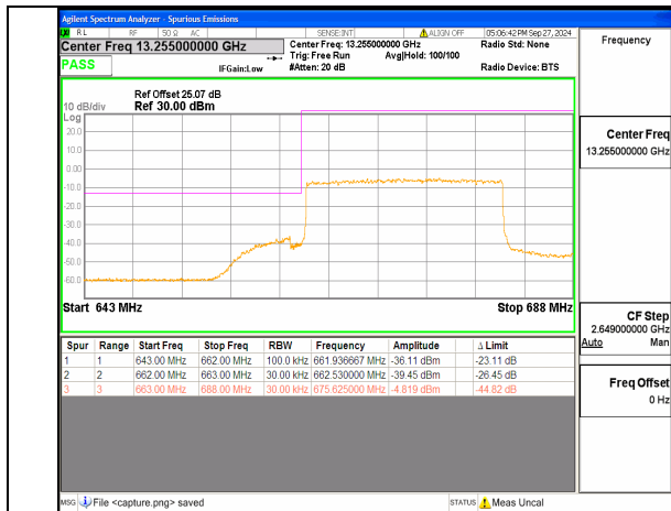
n71 20M DFT-s-OFDM BPSK Outer_Full Low
