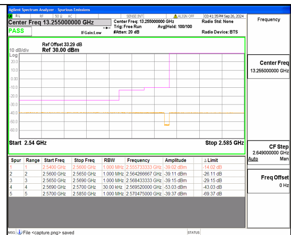
n38 10M DFT-s-OFDM BPSK Edge_1RB_Left Low
