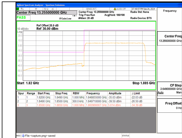
n25 30M DFT-s-OFDM QPSK Outer_Full Low
