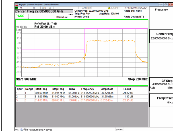
n26(814-824MHz) 5M DFT-s-OFDM QPSK Outer_Full Low
