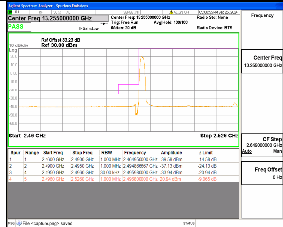
n41 30M DFT-s-OFDM QPSK Edge_1RB_Left Low
