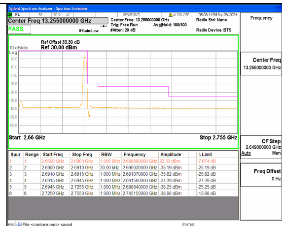
n41 30M DFT-s-OFDM QPSK Edge_1RB_Right High
