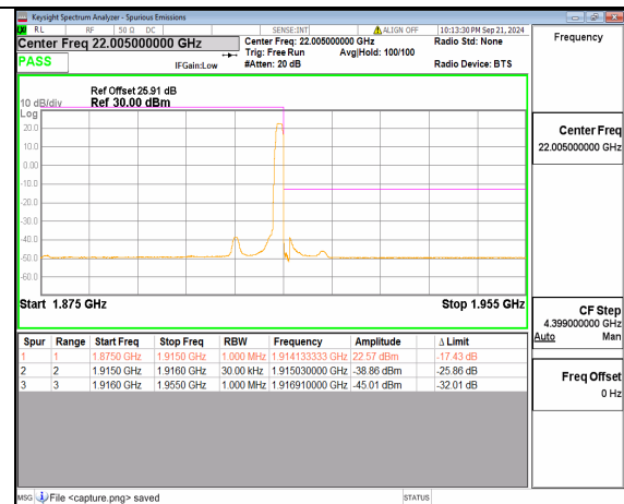
n25 40M DFT-s-OFDM BPSK Edge_1RB_Right High
