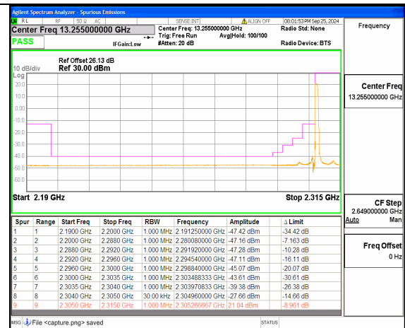
n30 10M DFT-s-OFDM BPSK Edge_1RB_Left Low
