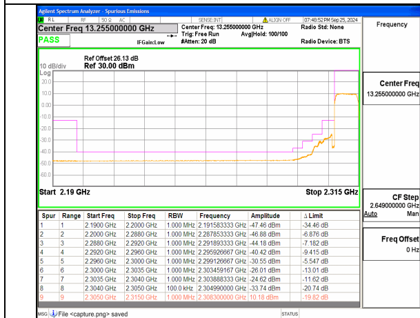
n30 10M DFT-s-OFDM QPSK Outer_Full Low
