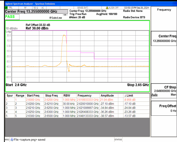
n38 15M DFT-s-OFDM QPSK Edge_1RB_Right High
