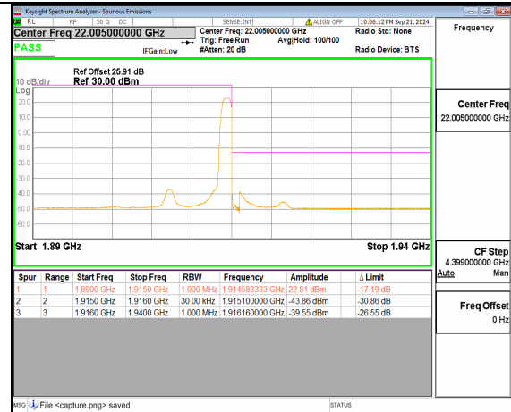
n25 25M DFT-s-OFDM BPSK Edge_1RB_Right High
