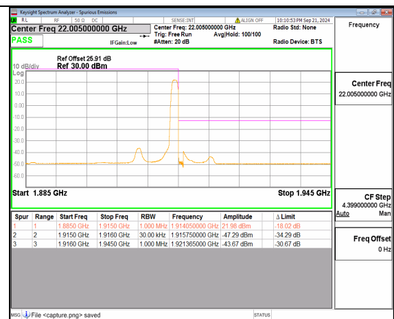
n25 30M DFT-s-OFDM QPSK Edge_1RB_Right High
