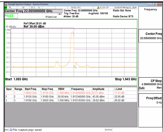
n25 30M DFT-s-OFDM BPSK Edge_1RB_Right High
