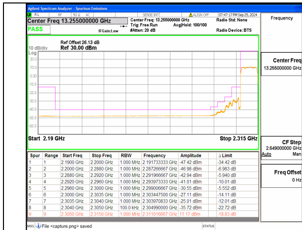
n30 10M DFT-s-OFDM BPSK Outer_Full Low
