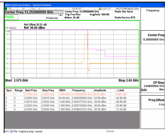
n38 40M DFT-s-OFDM BPSK Edge_1RB_Right High
