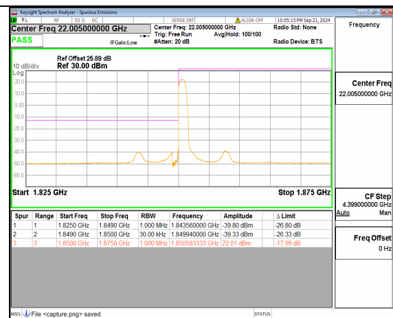
n25 25M DFT-s-OFDM QPSK Edge_1RB_Left Low
