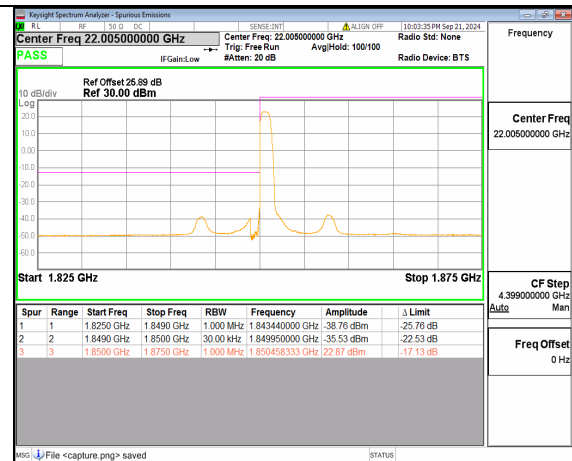
n25 25M DFT-s-OFDM BPSK Edge_1RB_Left Low
