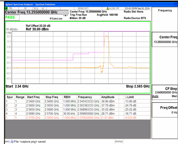
n38 10M DFT-s-OFDM QPSK Edge_1RB_Left Low
