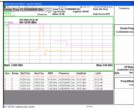
n38 10M DFT-s-OFDM BPSK Edge_1RB_Right High
