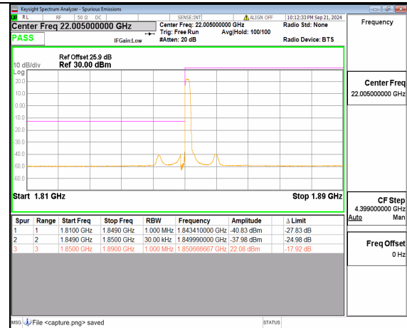
n25 40M DFT-s-OFDM QPSK Edge_1RB_Left Low
