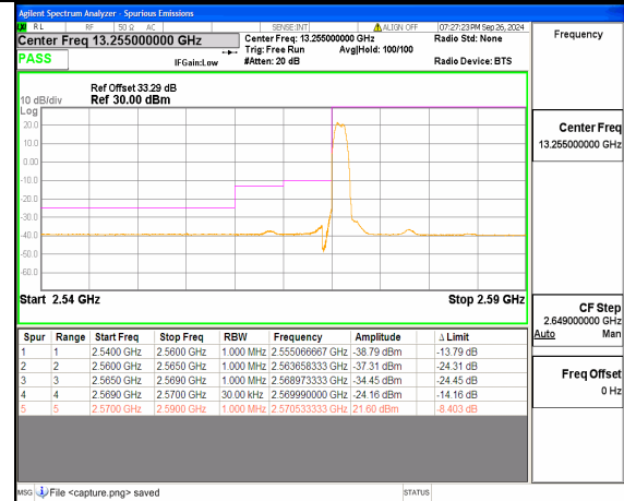
n38 15M DFT-s-OFDM BPSK Edge_1RB_Left Low
