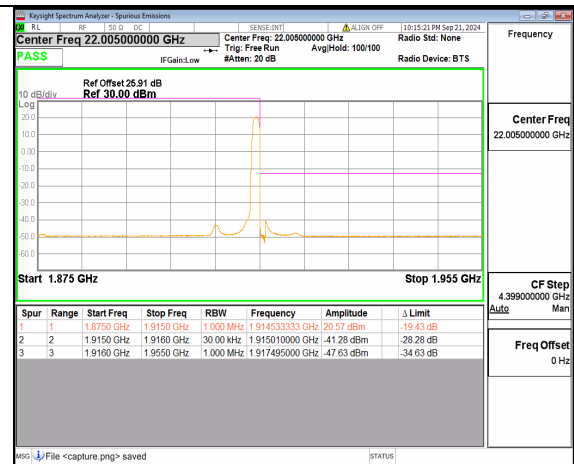
n25 40M DFT-s-OFDM QPSK Edge_1RB_Right High
