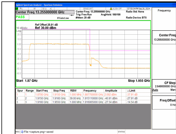
n25 40M DFT-s-OFDM QPSK Outer_Full High
