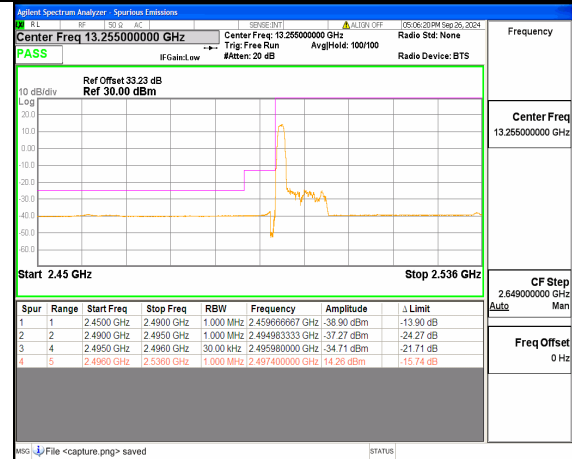
n41 40M DFT-s-OFDM BPSK Edge_1RB_Left Low
