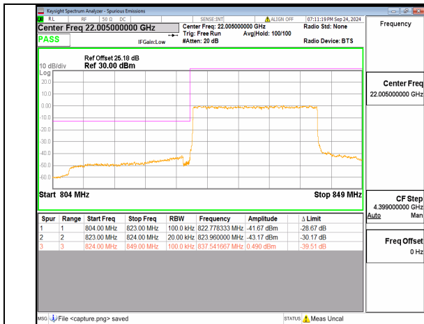
n26(824-849MHz) 20M DFT-s-OFDM QPSK Outer_Full Low
