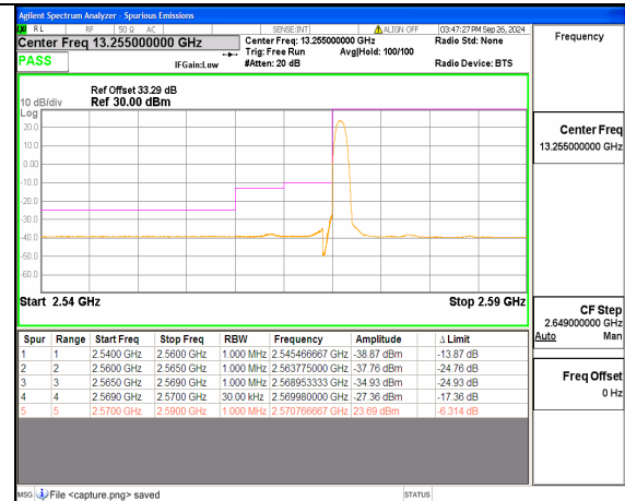
n38 15M DFT-s-OFDM QPSK Edge_1RB_Left Low
