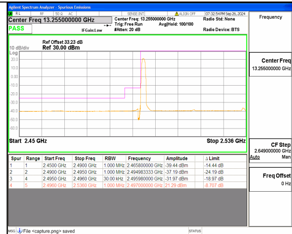
n41 40M DFT-s-OFDM QPSK Edge_1RB_Left Low
