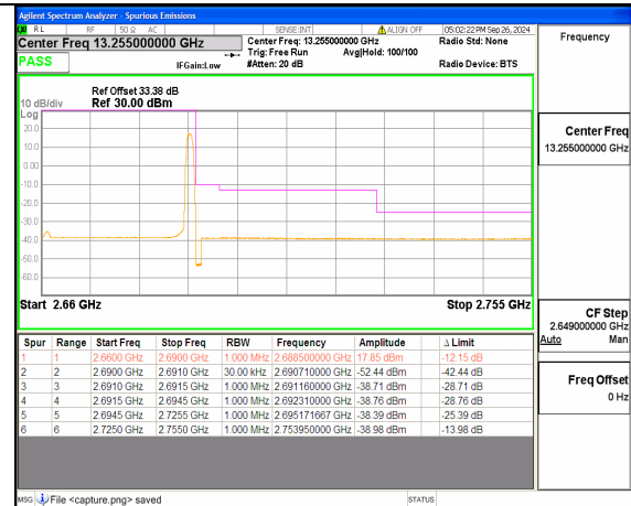
n41 30M DFT-s-OFDM BPSK Edge_1RB_Right High
