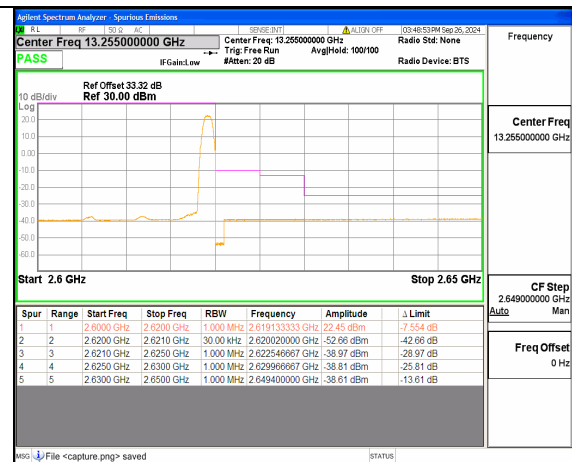
n38 15M DFT-s-OFDM BPSK Edge_1RB_Right High
