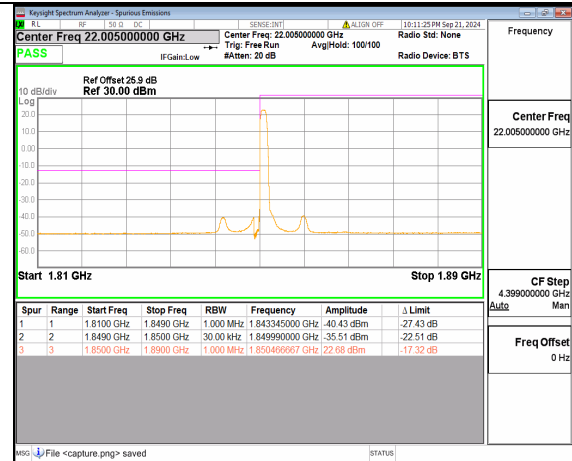
n25 40M DFT-s-OFDM BPSK Edge_1RB_Left Low
