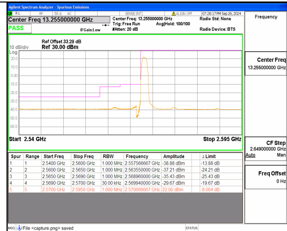
n38 20M DFT-s-OFDM BPSK Edge_1RB_Left Low
