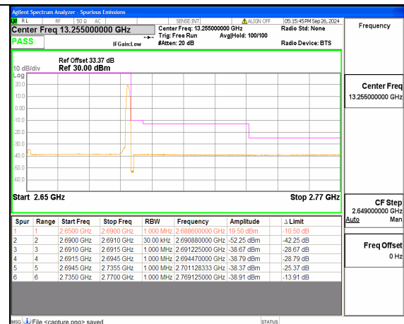
n41 40M DFT-s-OFDM BPSK Edge_1RB_Right High
