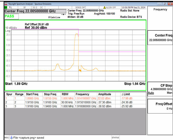
n25 25M DFT-s-OFDM QPSK Edge_1RB_Right High
