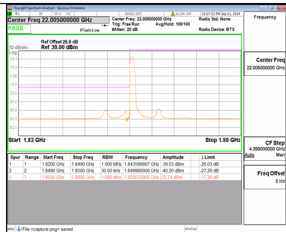
n25 30M DFT-s-OFDM BPSK Edge_1RB_Left Low
