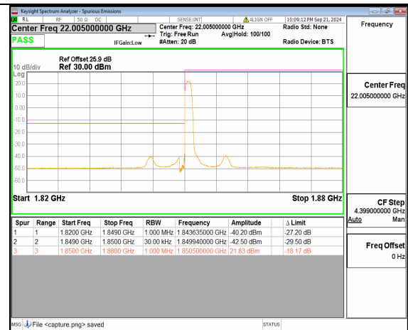
n25 30M DFT-s-OFDM QPSK Edge_1RB_Left Low
