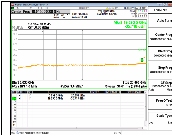
n78(3700-3800MHz) (30MHz-20GHz) 20M DFT-s-OFDM QPSK Inner_1RB_Right_High
