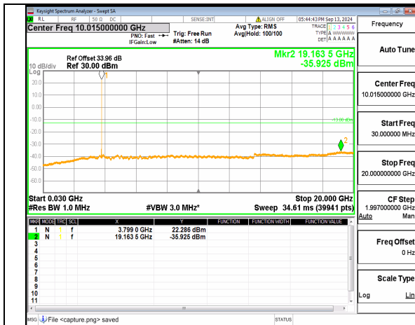
n78(3700-3800MHz) (30MHz-20GHz) 30M DFT-s-OFDM QPSK Inner_1RB_Right_High
