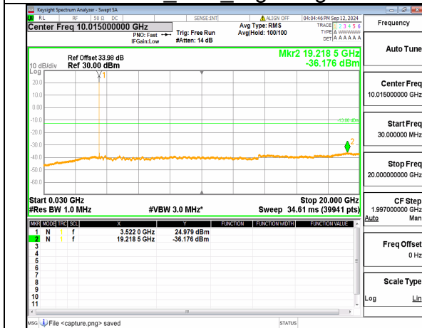
n78(3450-3550MHz) (30MHz-20GHz) 30M DFT-s-OFDM QPSK Inner_1RB_Left High
