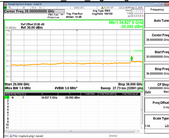
n78(3450-3550MHz) (20GHz-36GHz) 20M DFT-s-OFDM BPSK Inner_1RB_Left Low
