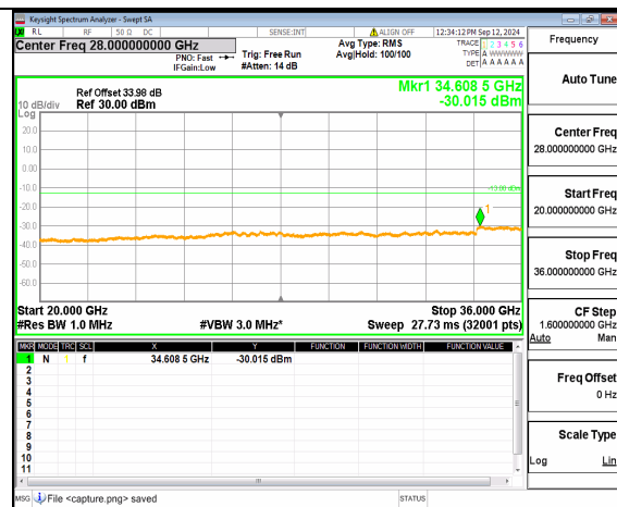
n78(3450-3550MHz) (20GHz-36GHz) 20M DFT-s-OFDM BPSK Inner_1RB_Right Mid
