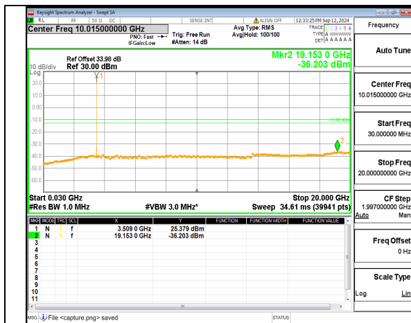
n78(3450-3550MHz) (30MHz-20GHz) 20M DFT-s-OFDM BPSK Inner_1RB_Right Mid
