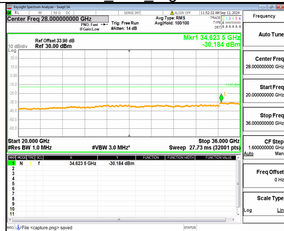
n78(3450-3550MHz) (20GHz-36GHz) 15M DFT-s-OFDM BPSK Inner_1RB_Left Mid
